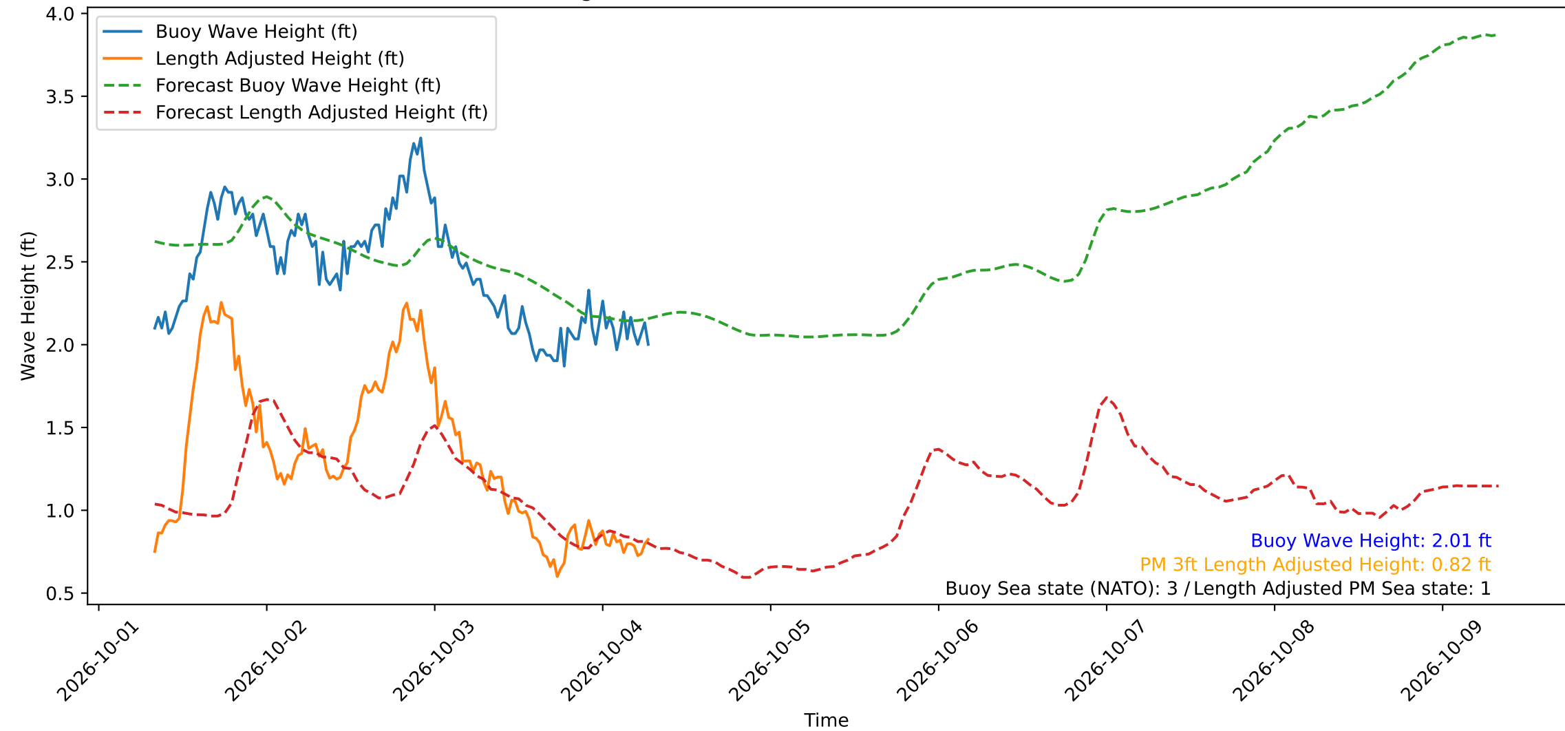
Wave Heights over Time for Red Beach at 2026-10-04 07:30:50
