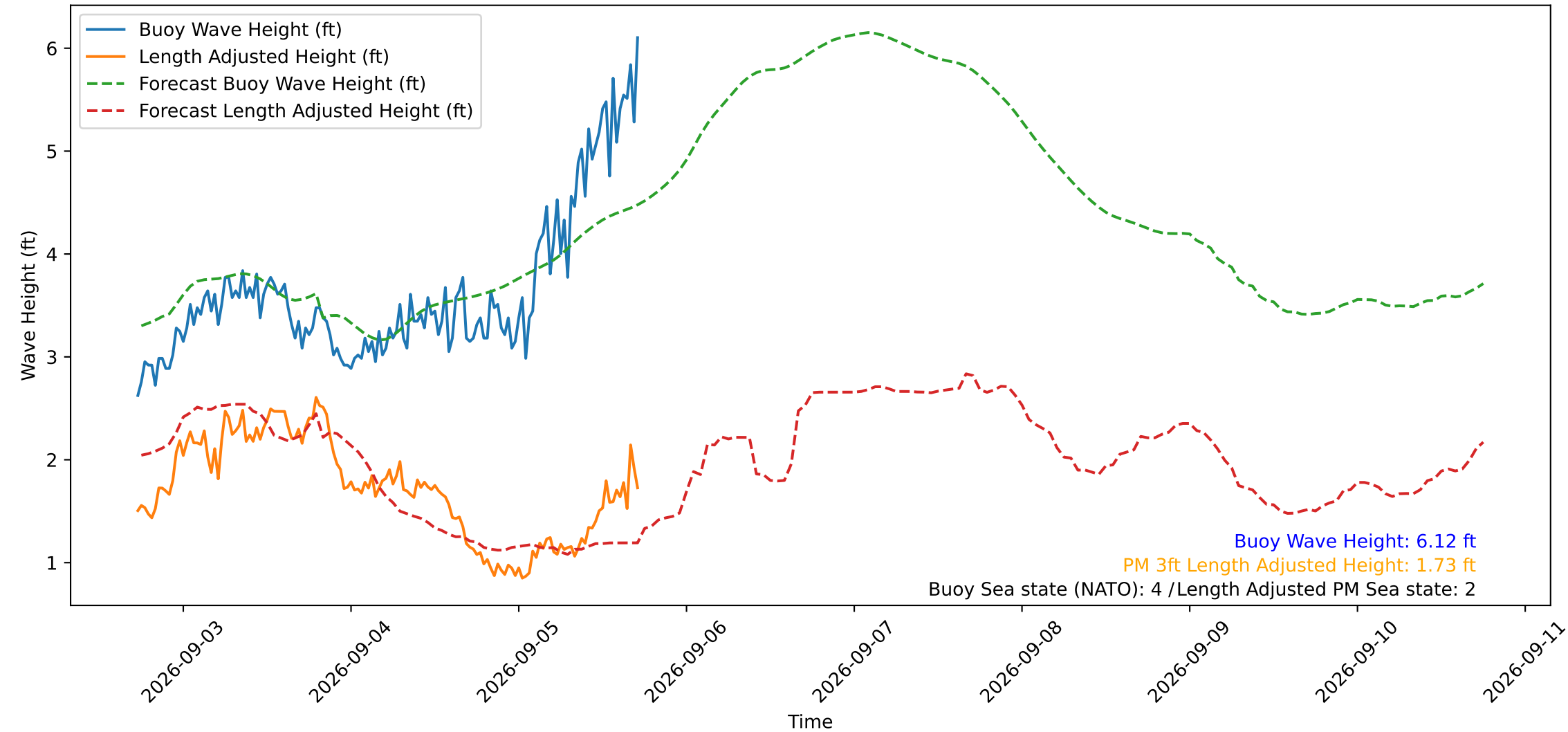
Wave Heights over Time for Oceanside Harbor at 2026-09-05 17:40:30
