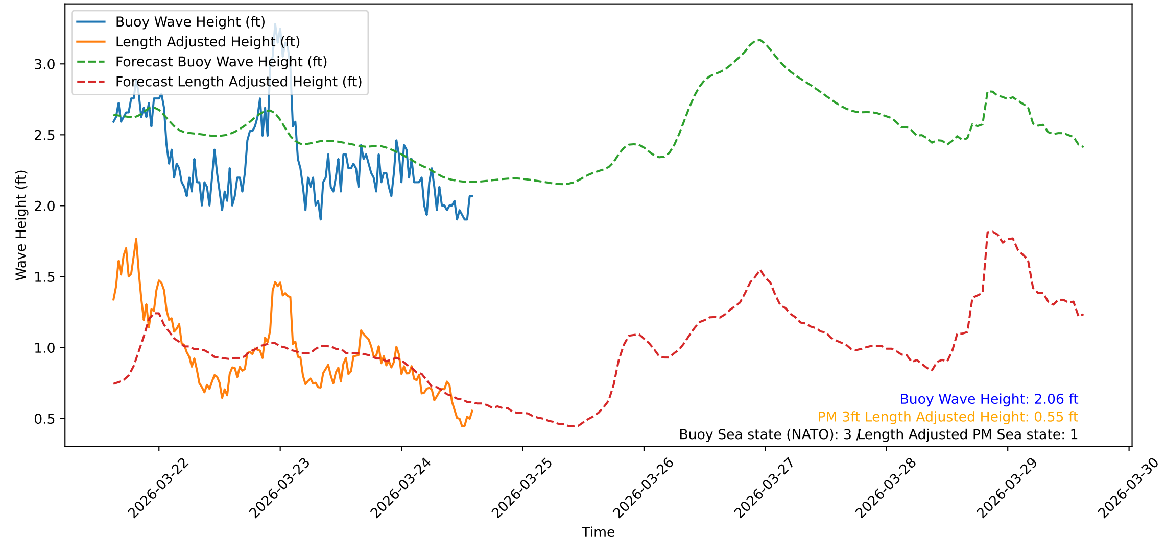
Wave Heights over Time for Green Beach at 2026-03-24 15:01:08
