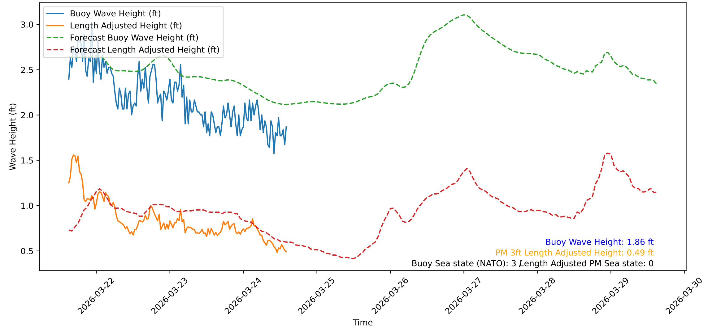
Wave Heights over Time for Oceanside Harbor at 2026-03-24 15:00:31
