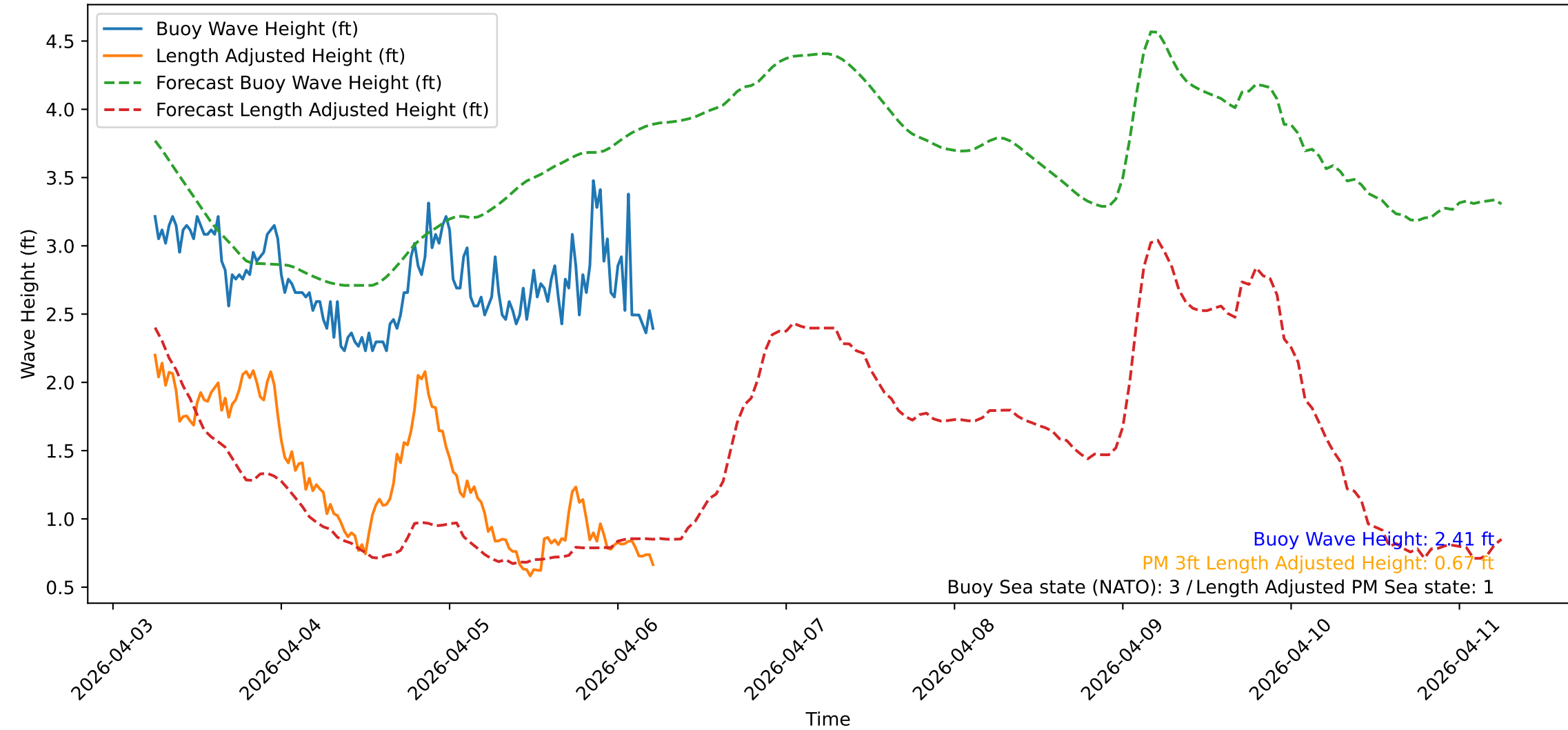
Wave Heights over Time for Green Beach at 2026-04-06 05:51:09
