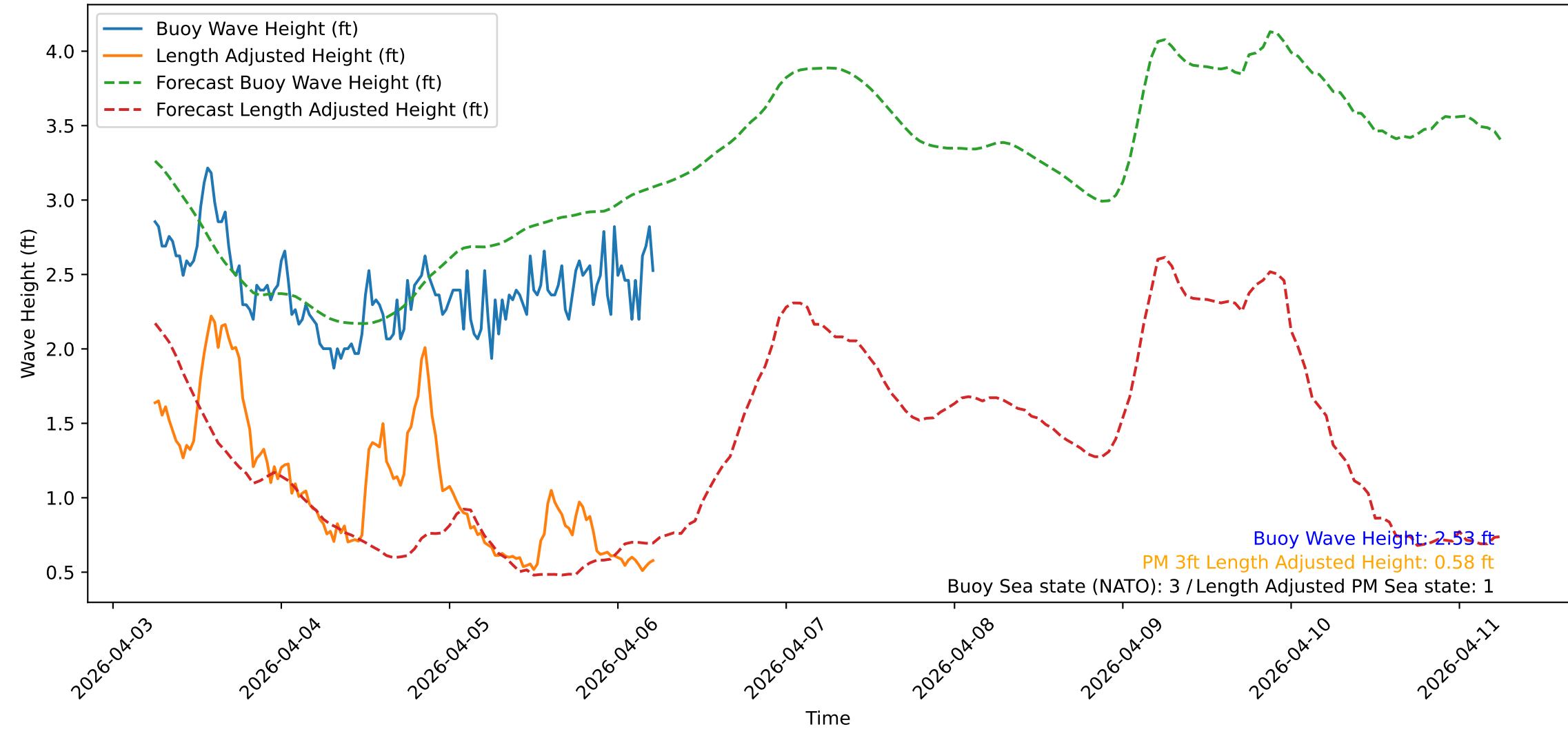
Wave Heights over Time for Red Beach at 2026-04-06 05:50:47
