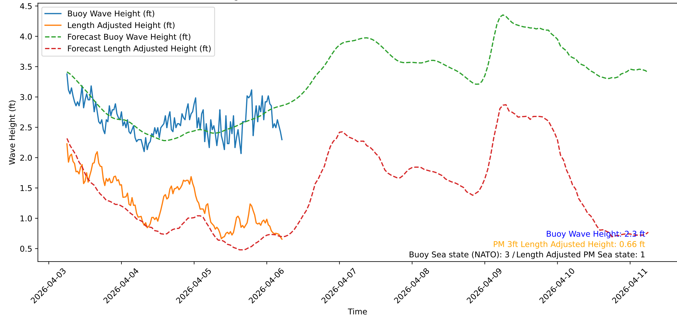
Wave Heights over Time for Oceanside Harbor at 2026-04-06 05:50:31
