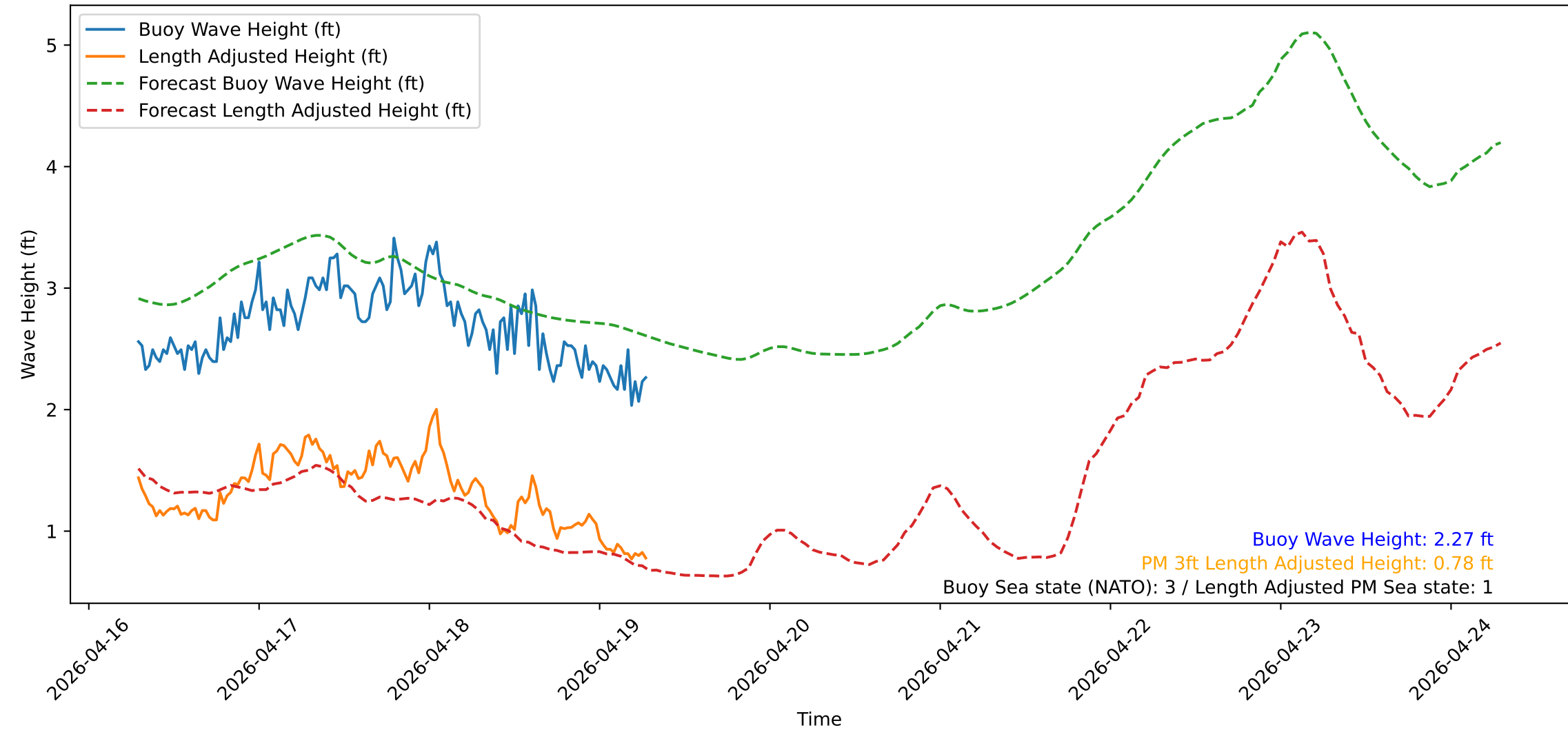
Wave Heights over Time for Oceanside Harbor at 2026-04-19 07:10:30
