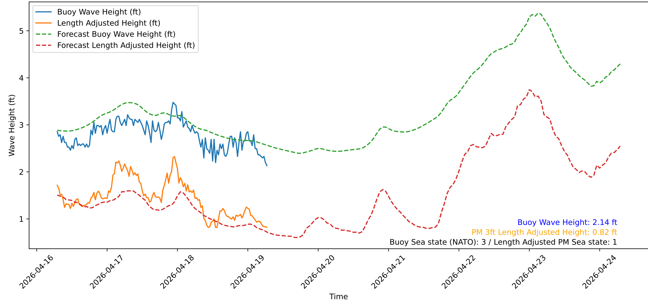
Wave Heights over Time for Green Beach at 2026-04-19 07:11:12
