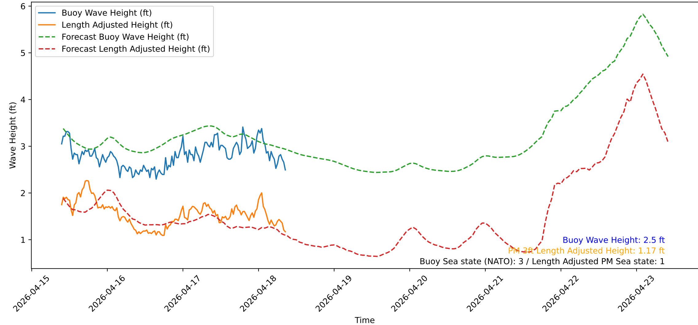
Wave Heights over Time for Oceanside Harbor at 2026-04-18 09:30:31
