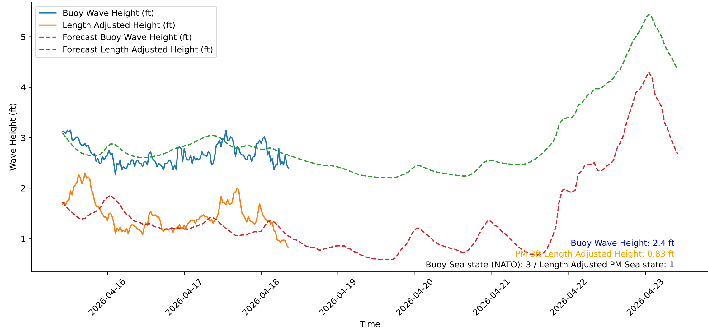
Wave Heights over Time for Red Beach at 2026-04-18 09:30:50
