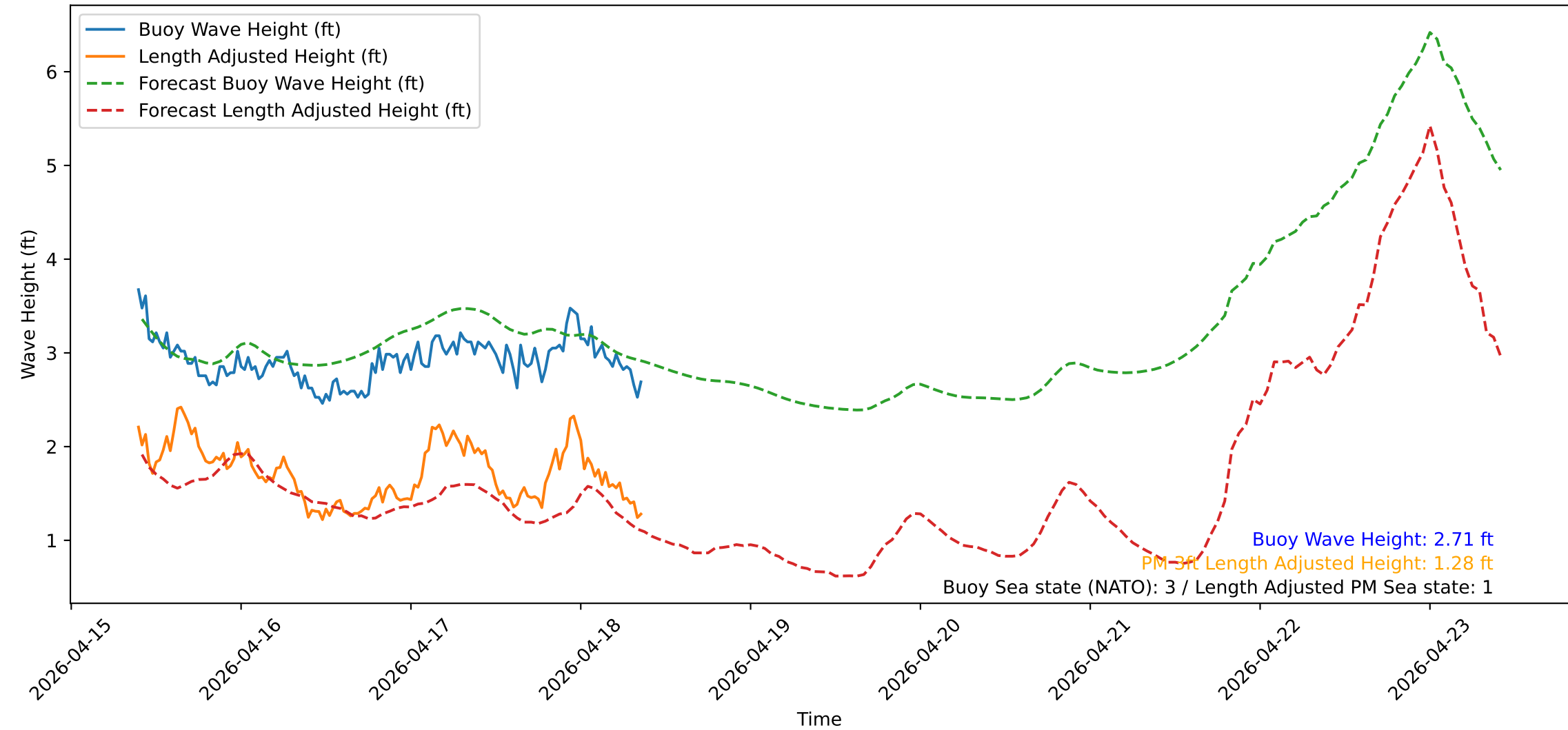
Wave Heights over Time for Green Beach at 2026-04-18 09:31:12
