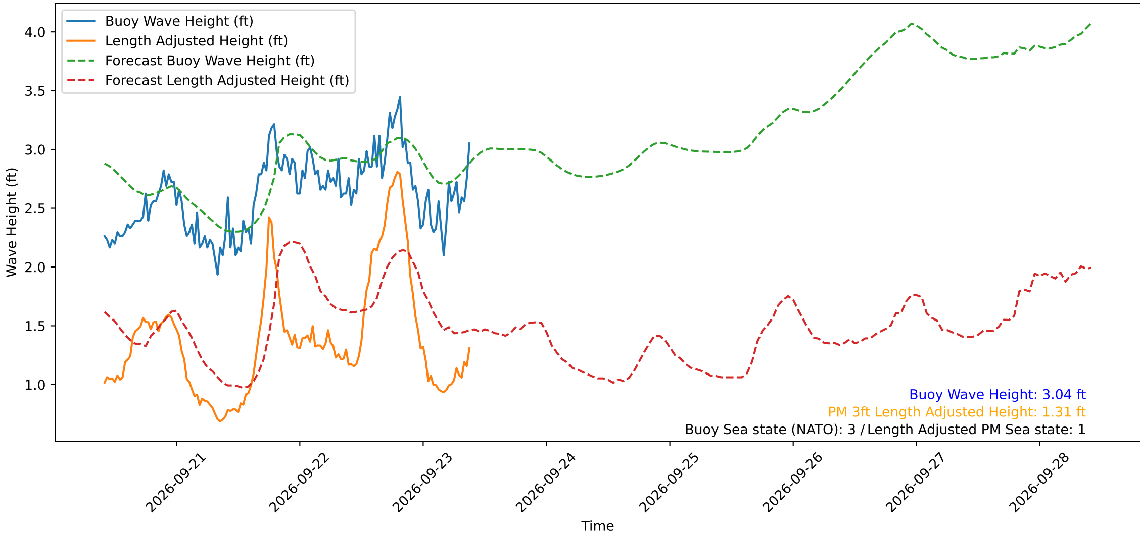
Wave Heights over Time for Green Beach at 2026-09-23 09:41:11
