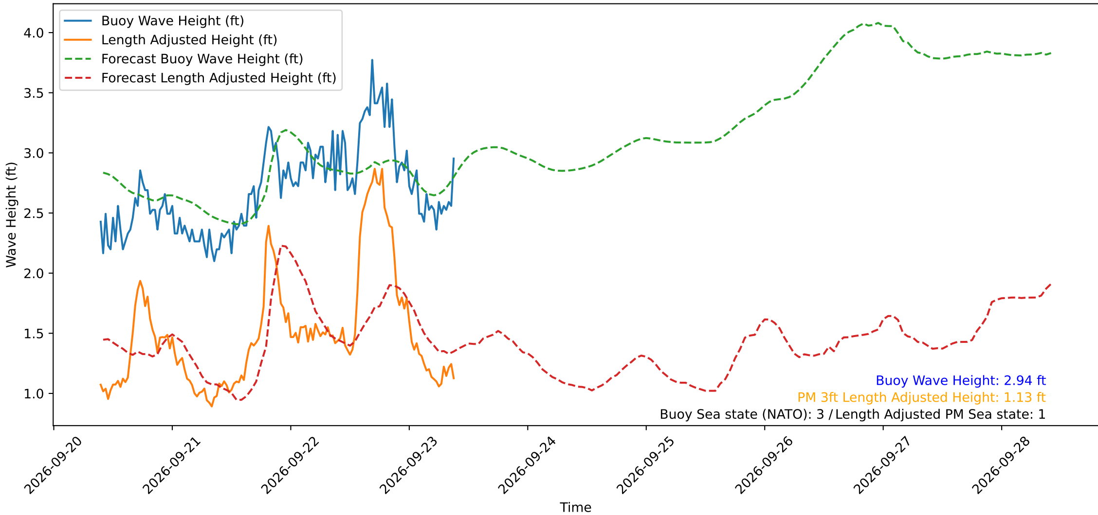
Wave Heights over Time for Oceanside Harbor at 2026-09-23 09:40:29
