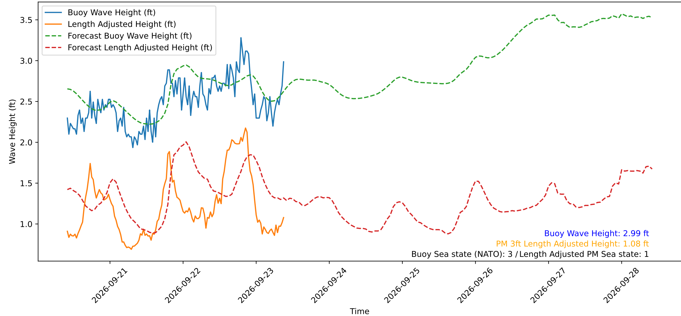
Wave Heights over Time for Red Beach at 2026-09-23 09:40:49
