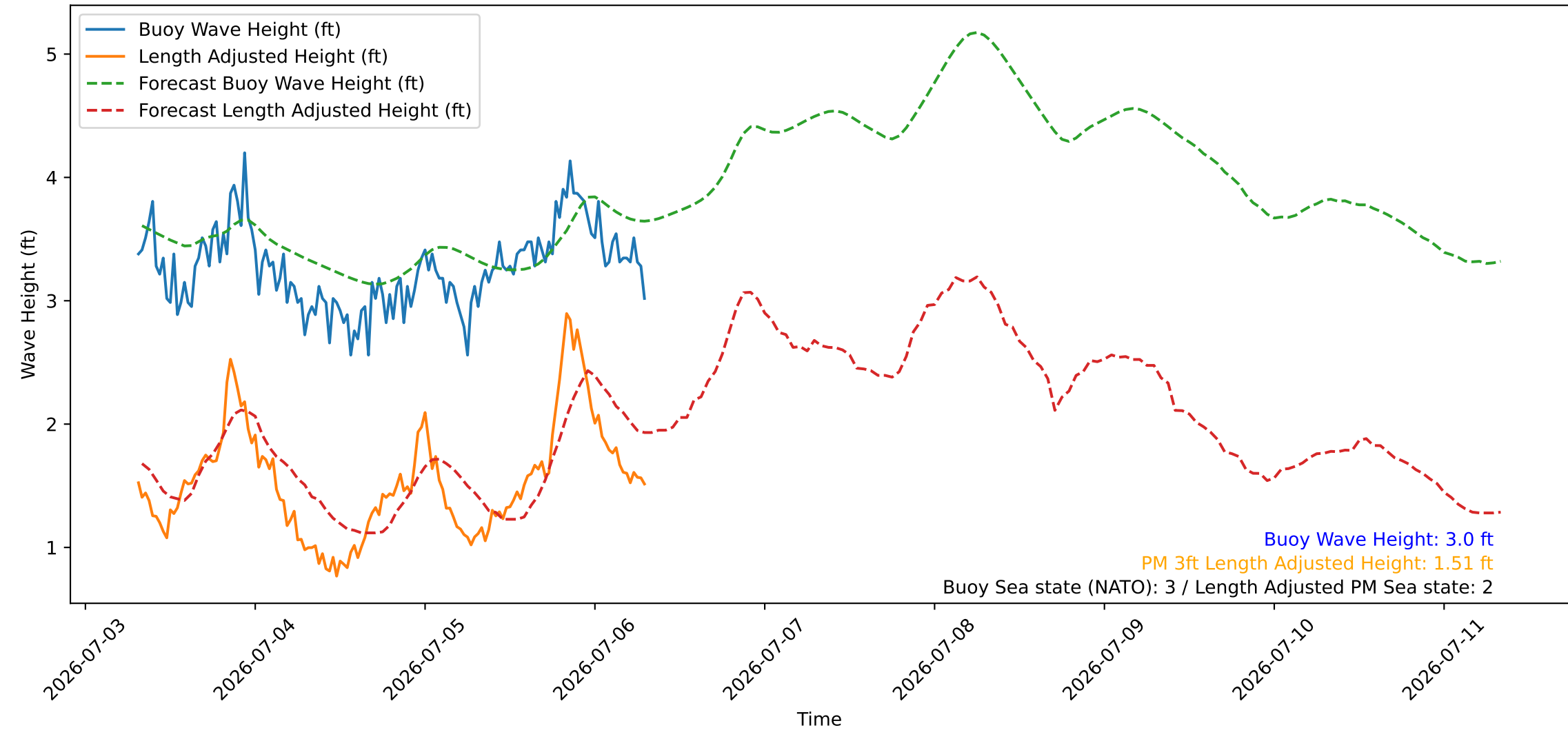
Wave Heights over Time for Green Beach at 2026-07-06 07:41:09
