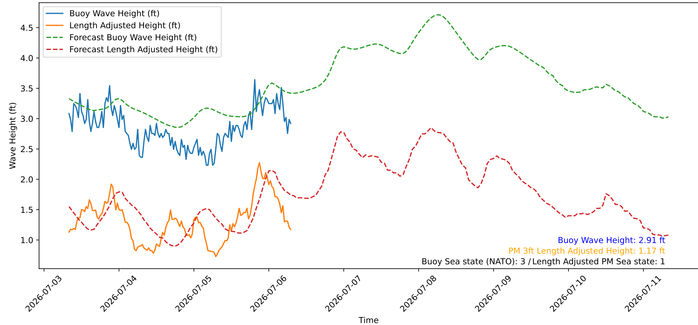
Wave Heights over Time for Red Beach at 2026-07-06 07:40:46
