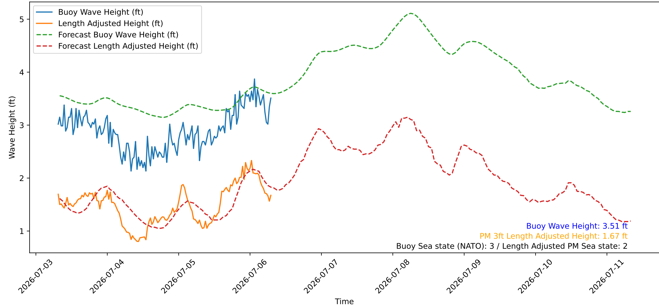
Wave Heights over Time for Oceanside Harbor at 2026-07-06 07:40:26
