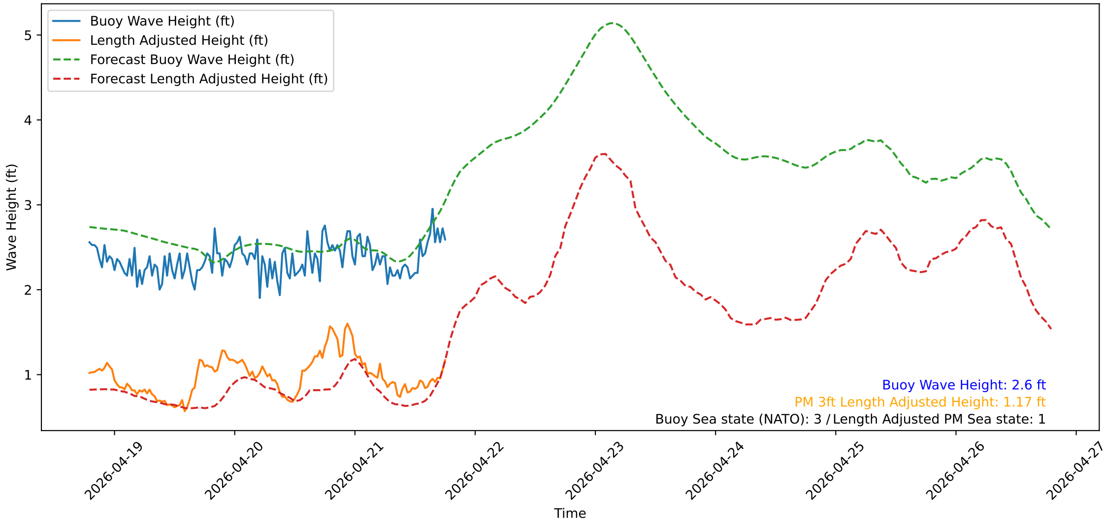
Wave Heights over Time for Oceanside Harbor at 2026-04-21 18:50:31
