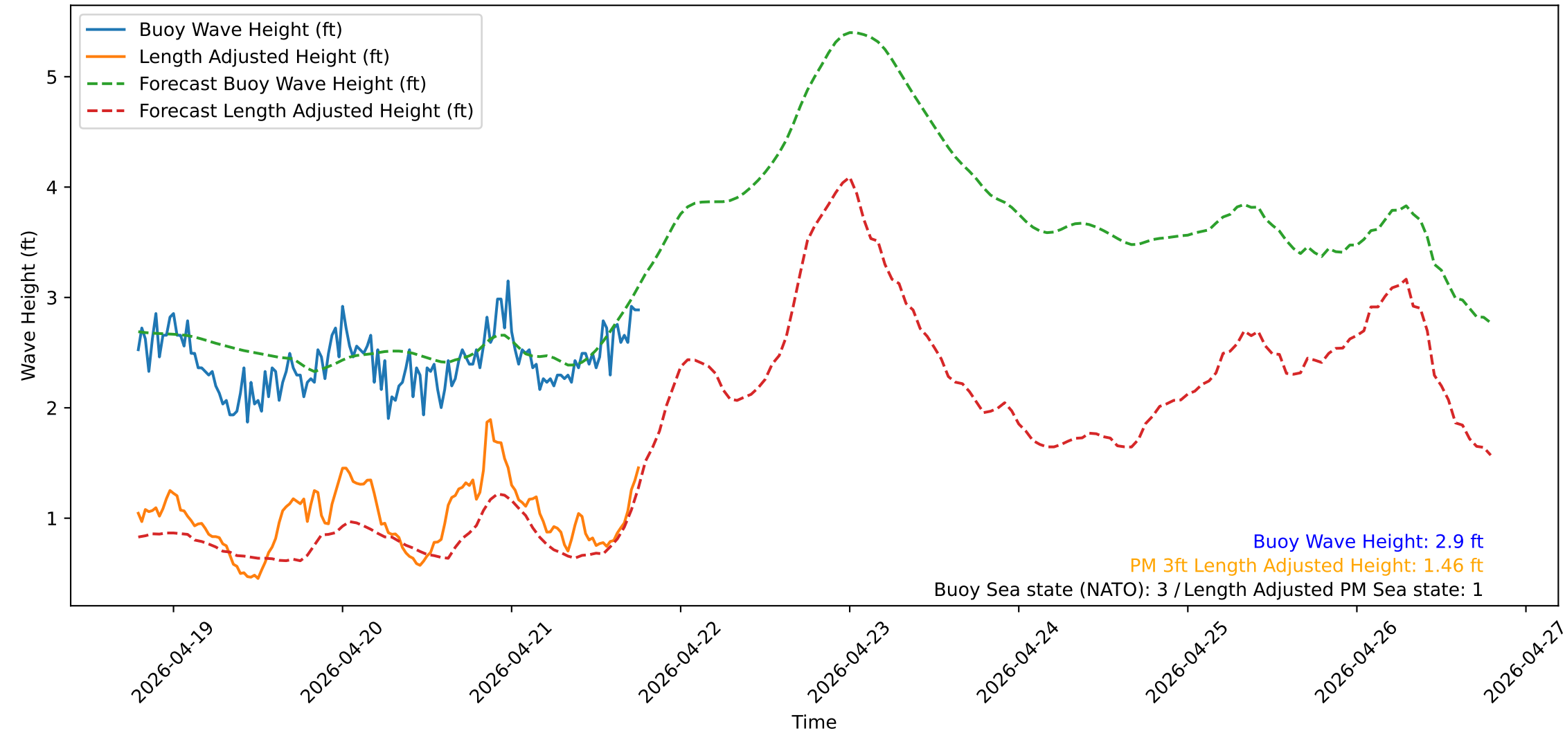
Wave Heights over Time for Green Beach at 2026-04-21 18:51:15
