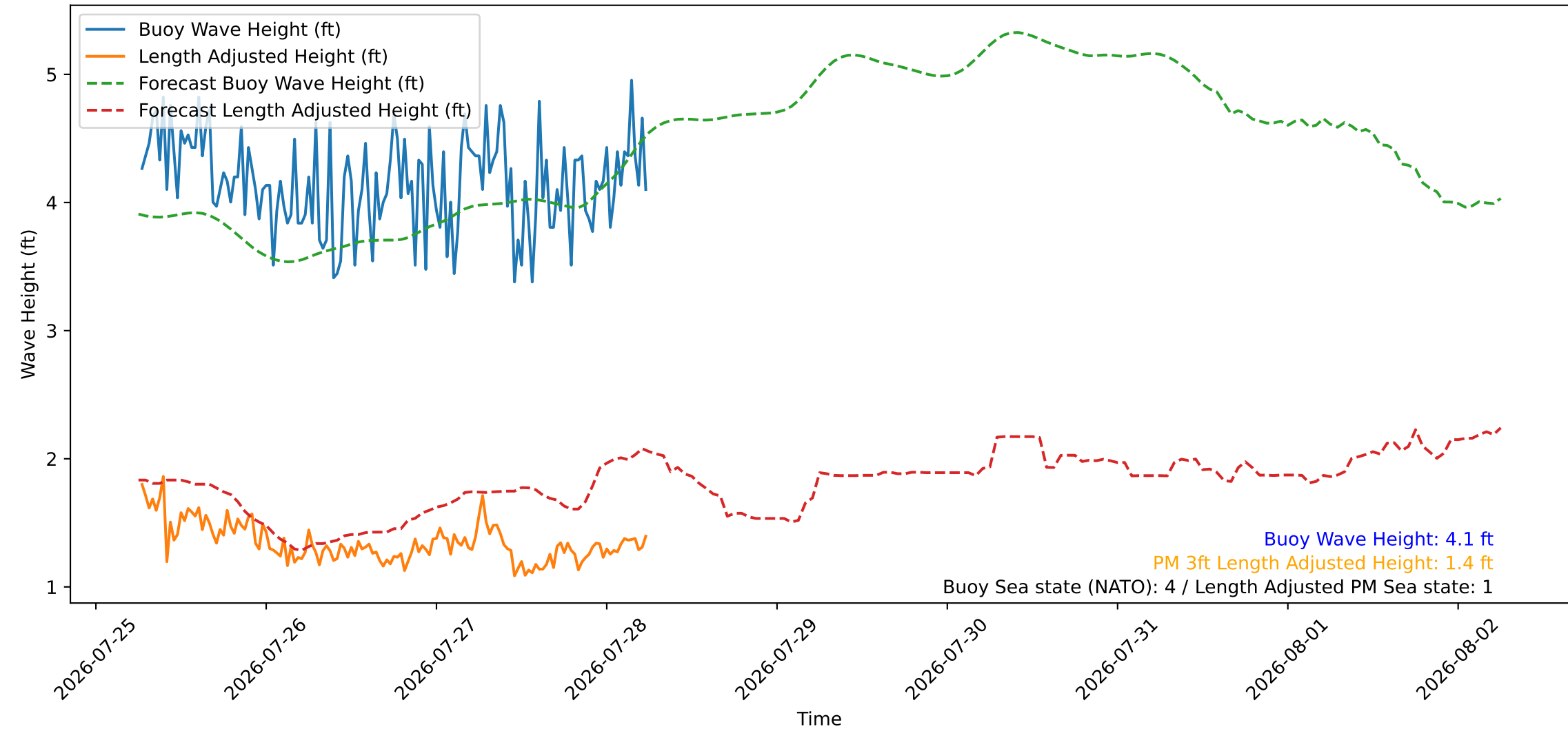
Wave Heights over Time for Green Beach at 2026-07-28 06:21:10
