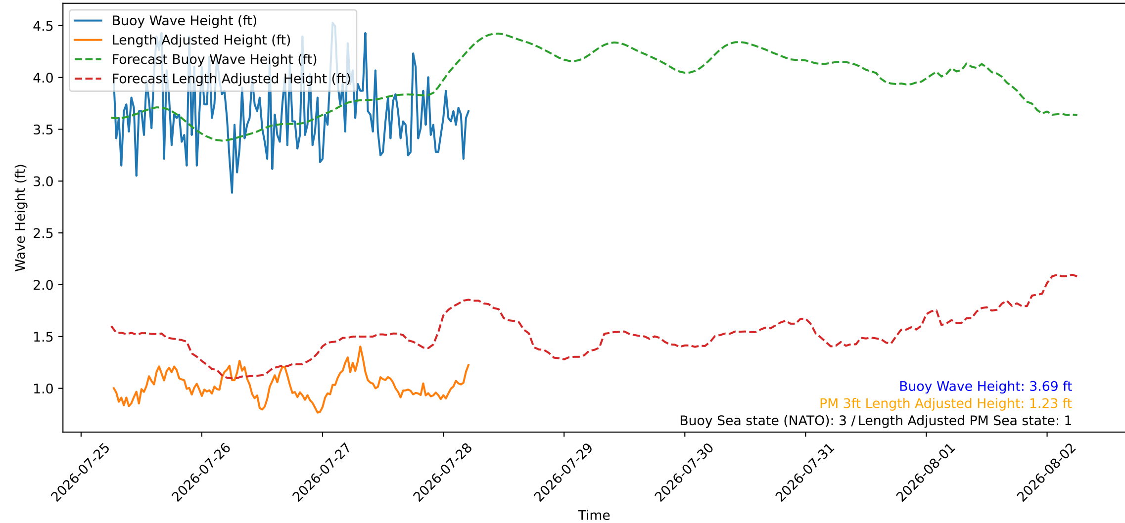
Wave Heights over Time for Red Beach at 2026-07-28 06:20:47
