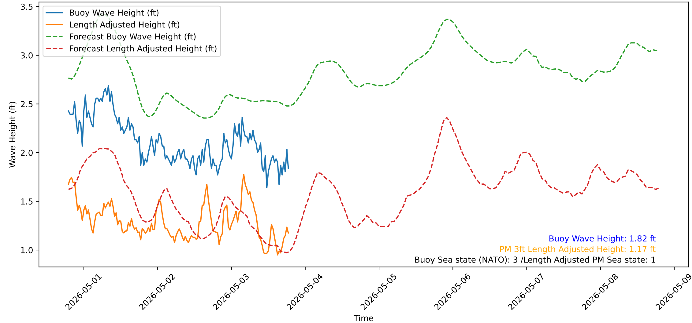
Wave Heights over Time for Oceanside Harbor at 2026-05-03 19:10:32
