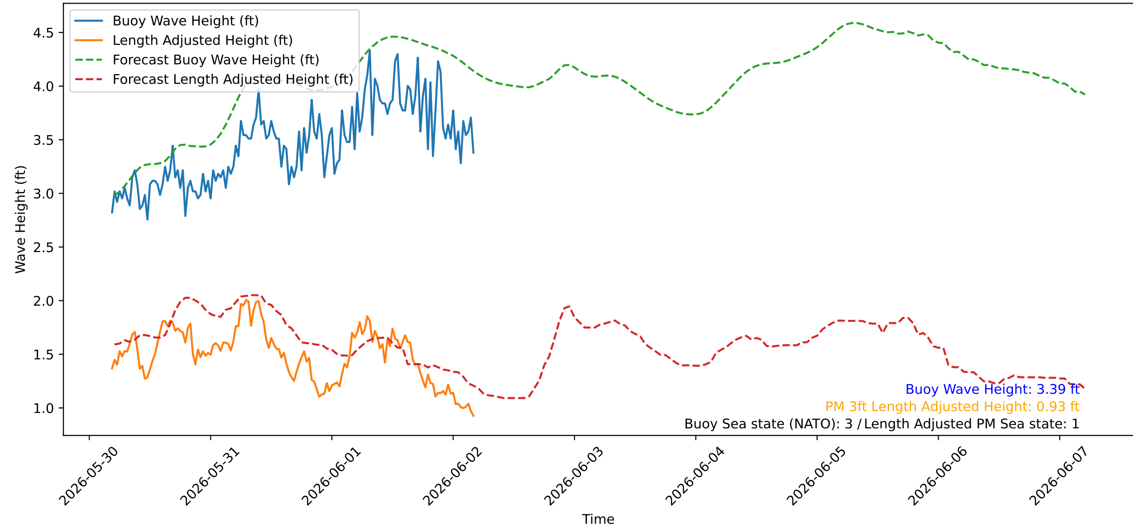
Wave Heights over Time for Green Beach at 2026-06-02 04:41:07
