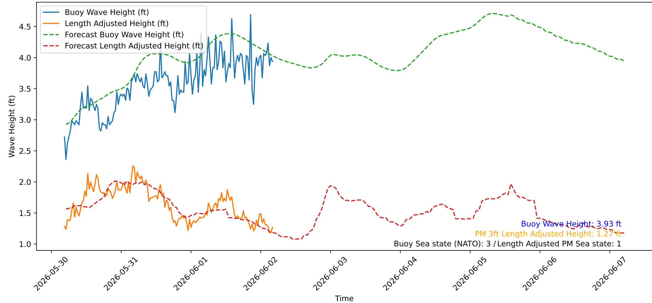
Wave Heights over Time for Oceanside Harbor at 2026-06-02 04:40:26
