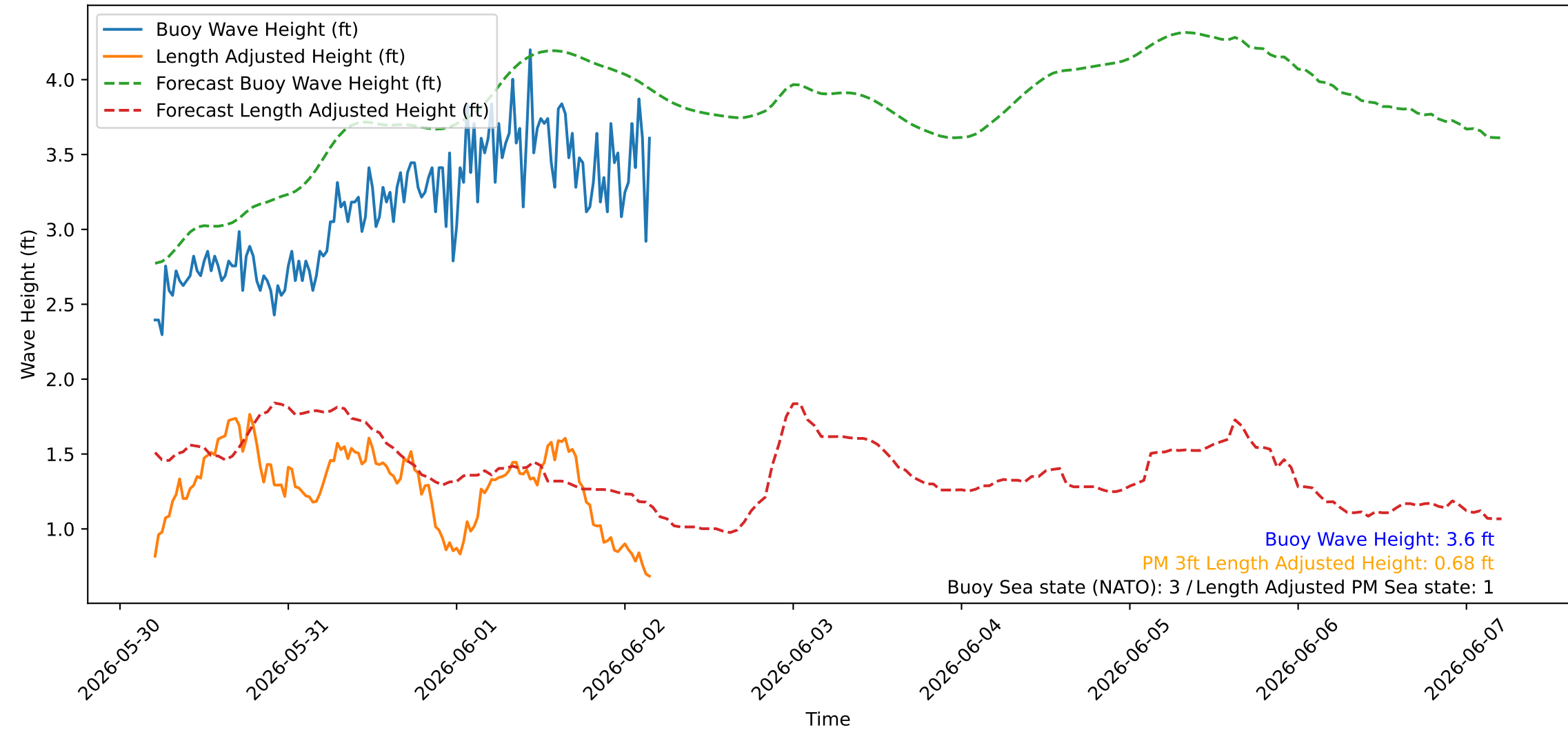
Wave Heights over Time for Red Beach at 2026-06-02 04:40:45
