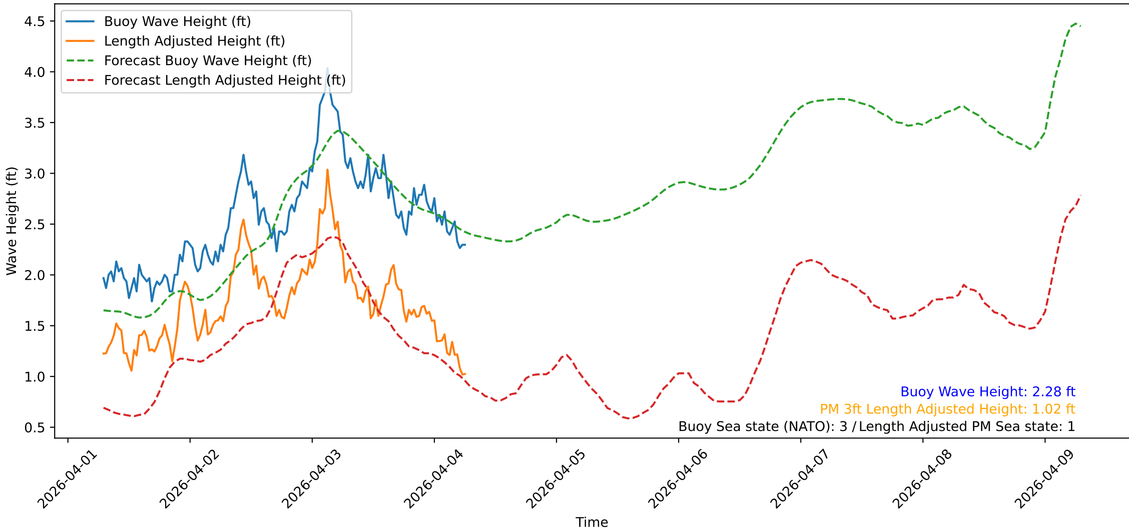
Wave Heights over Time for Oceanside Harbor at 2026-04-04 07:00:32
