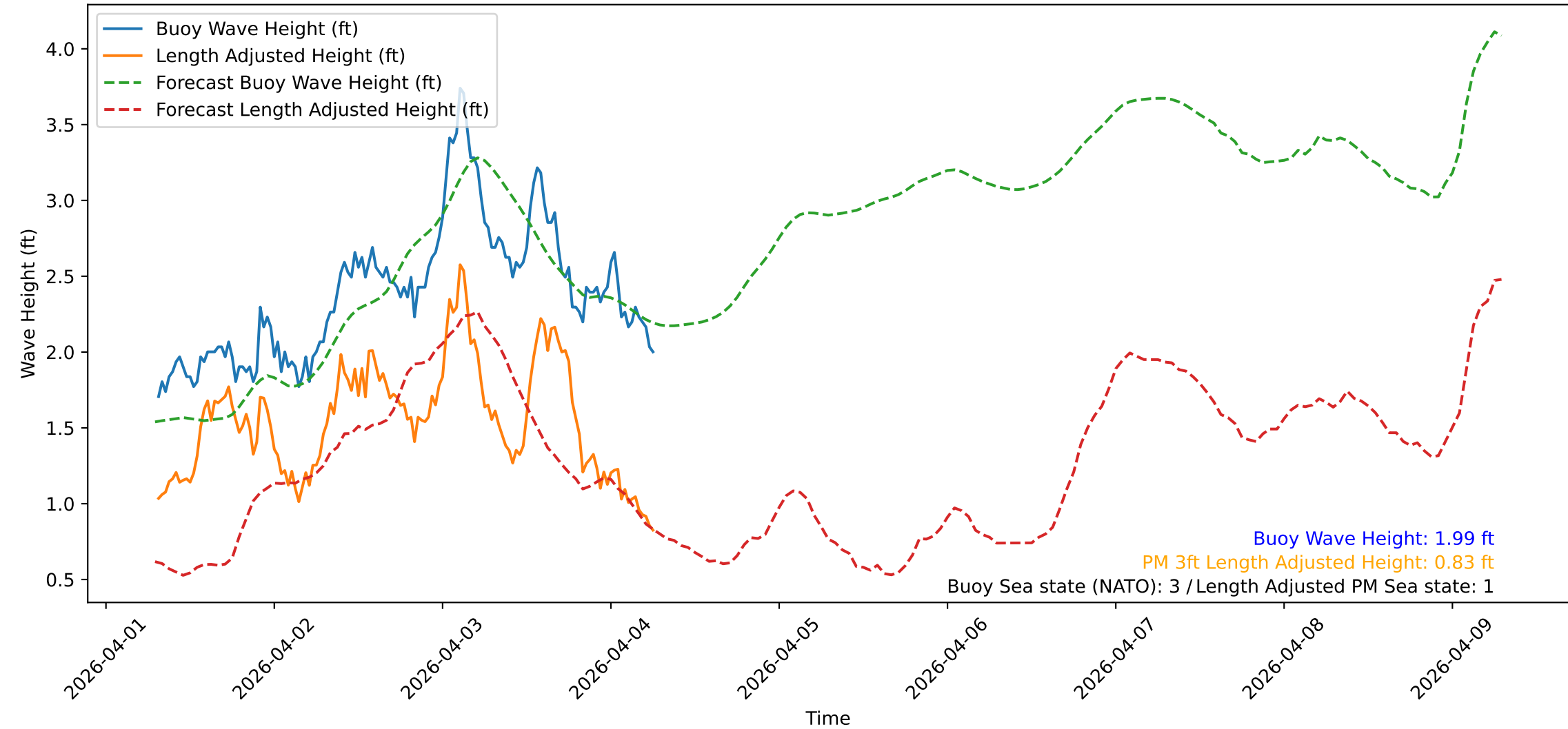
Wave Heights over Time for Red Beach at 2026-04-04 07:00:47
