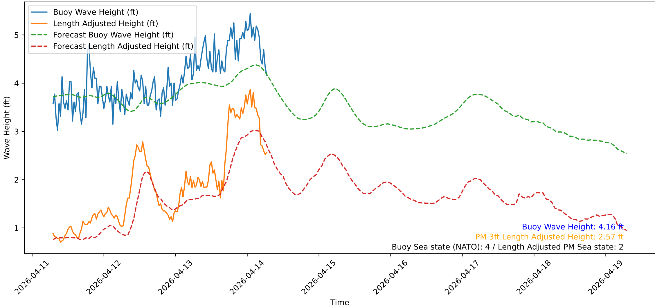
Wave Heights over Time for Oceanside Harbor at 2026-04-14 07:00:31
