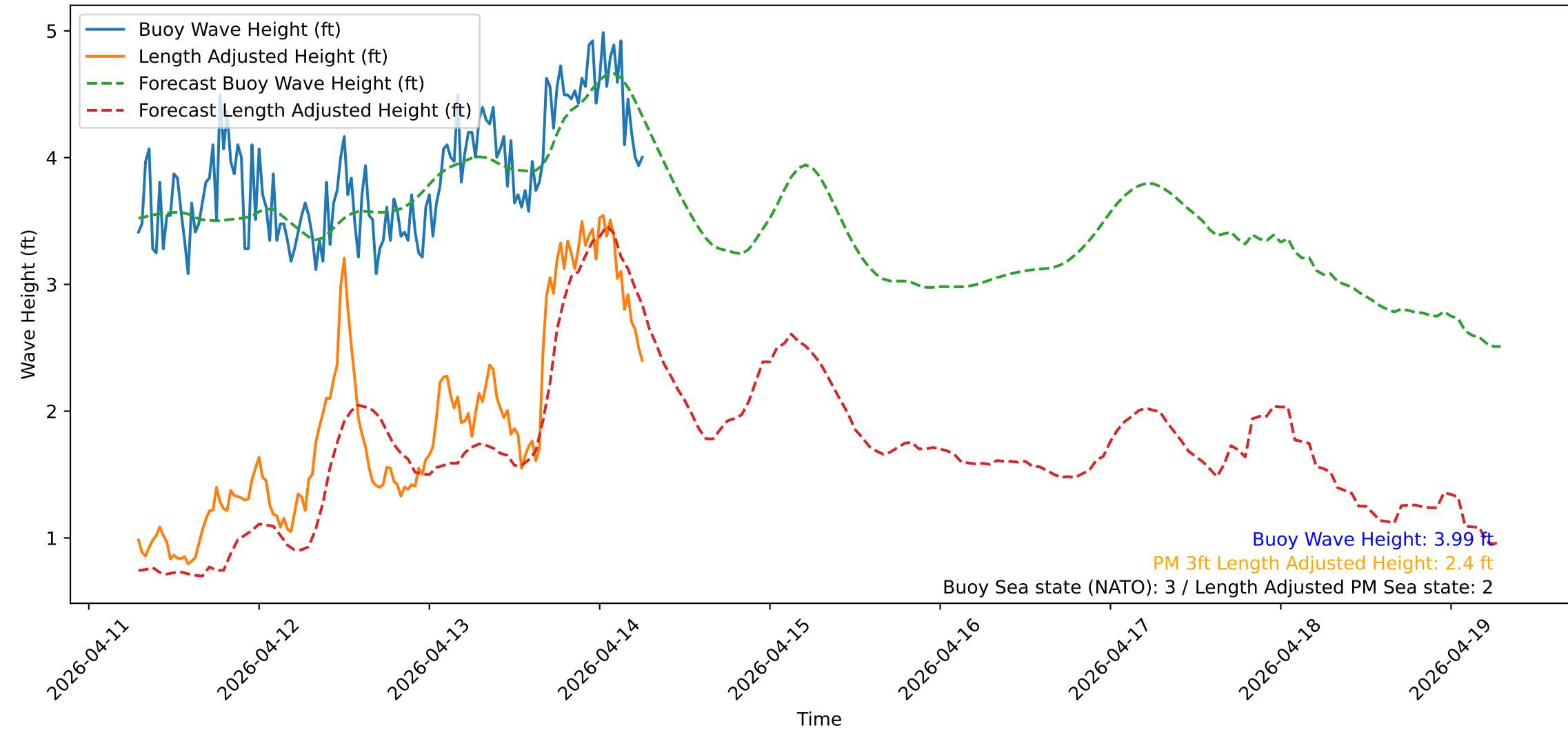
Wave Heights over Time for Green Beach at 2026-04-14 07:01:12
