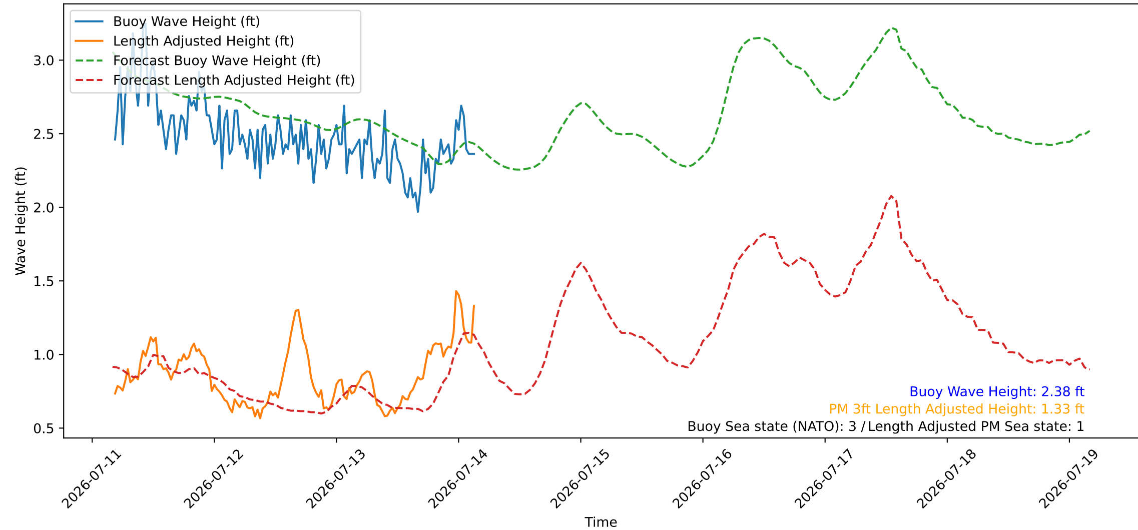
Wave Heights over Time for Red Beach at 2026-07-14 04:00:45
