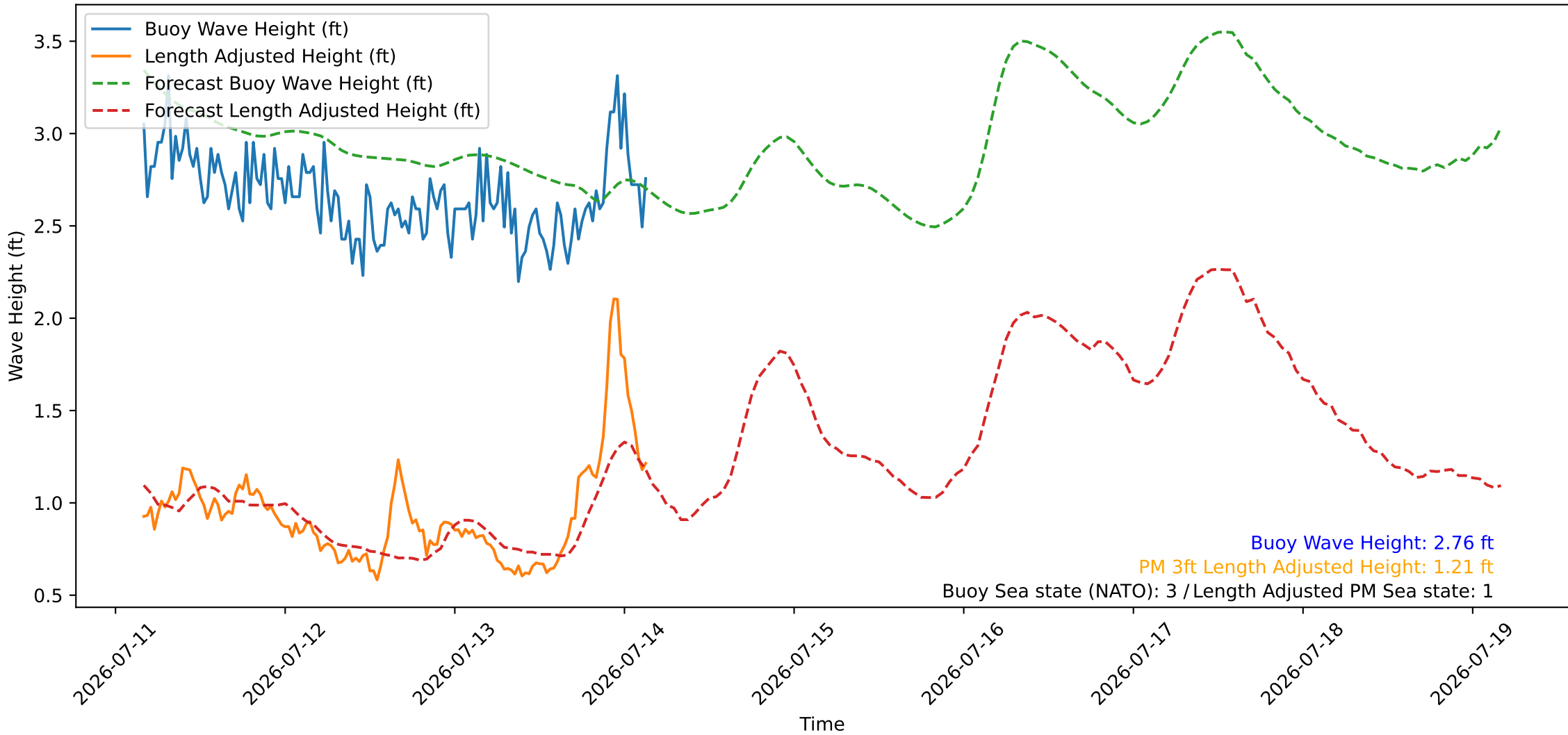
Wave Heights over Time for Green Beach at 2026-07-14 04:01:07
