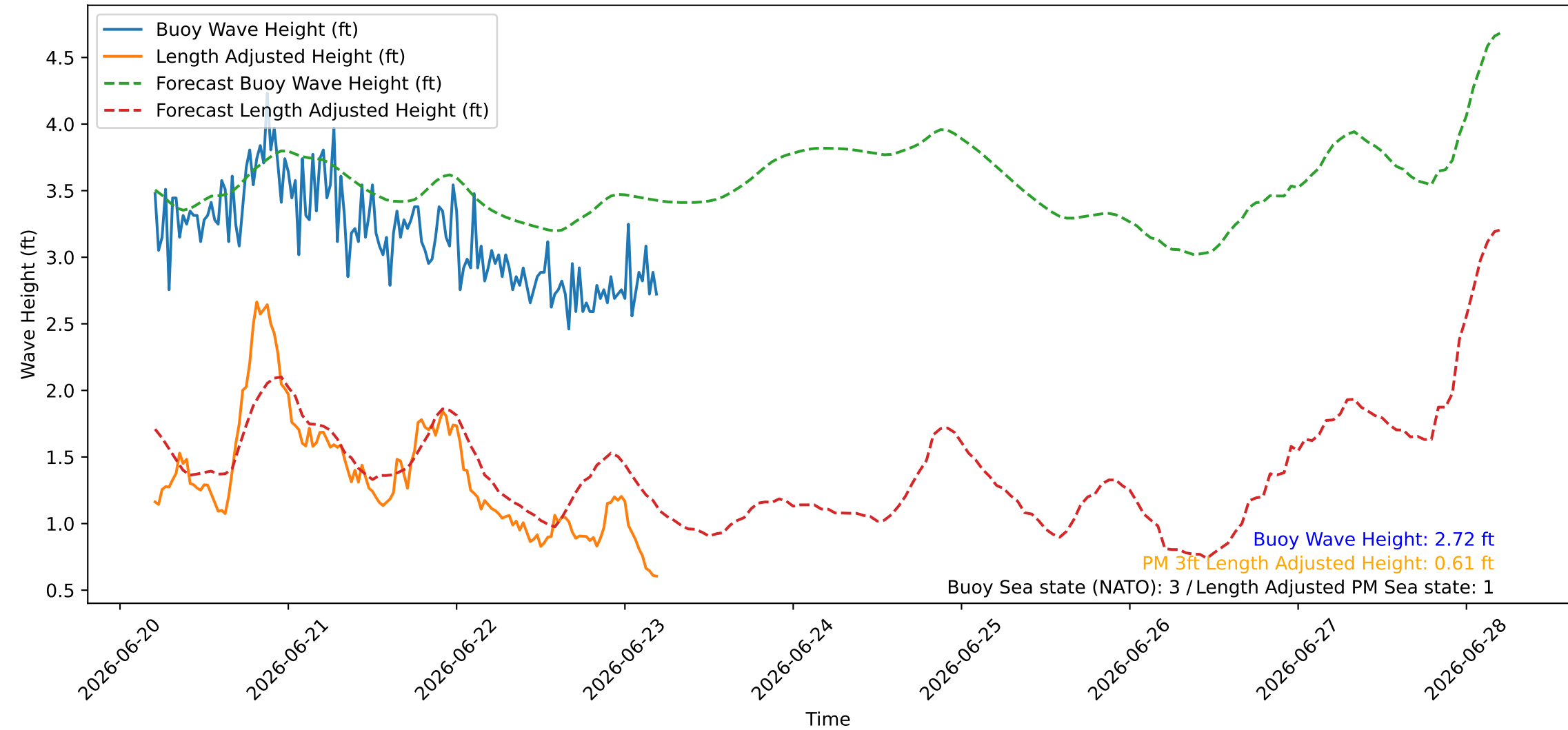
Wave Heights over Time for Green Beach at 2026-06-23 05:11:07
