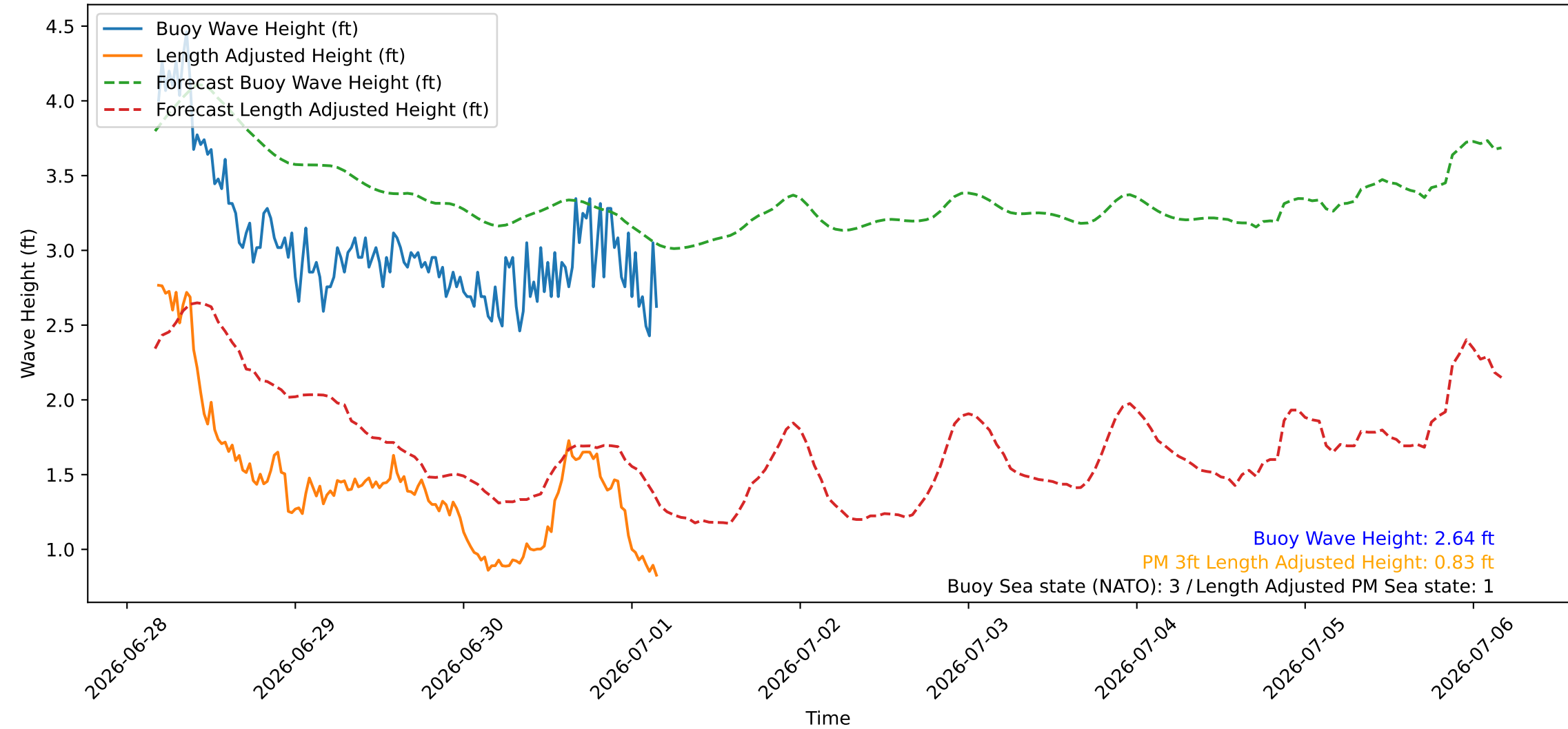
Wave Heights over Time for Red Beach at 2026-07-01 04:20:46
