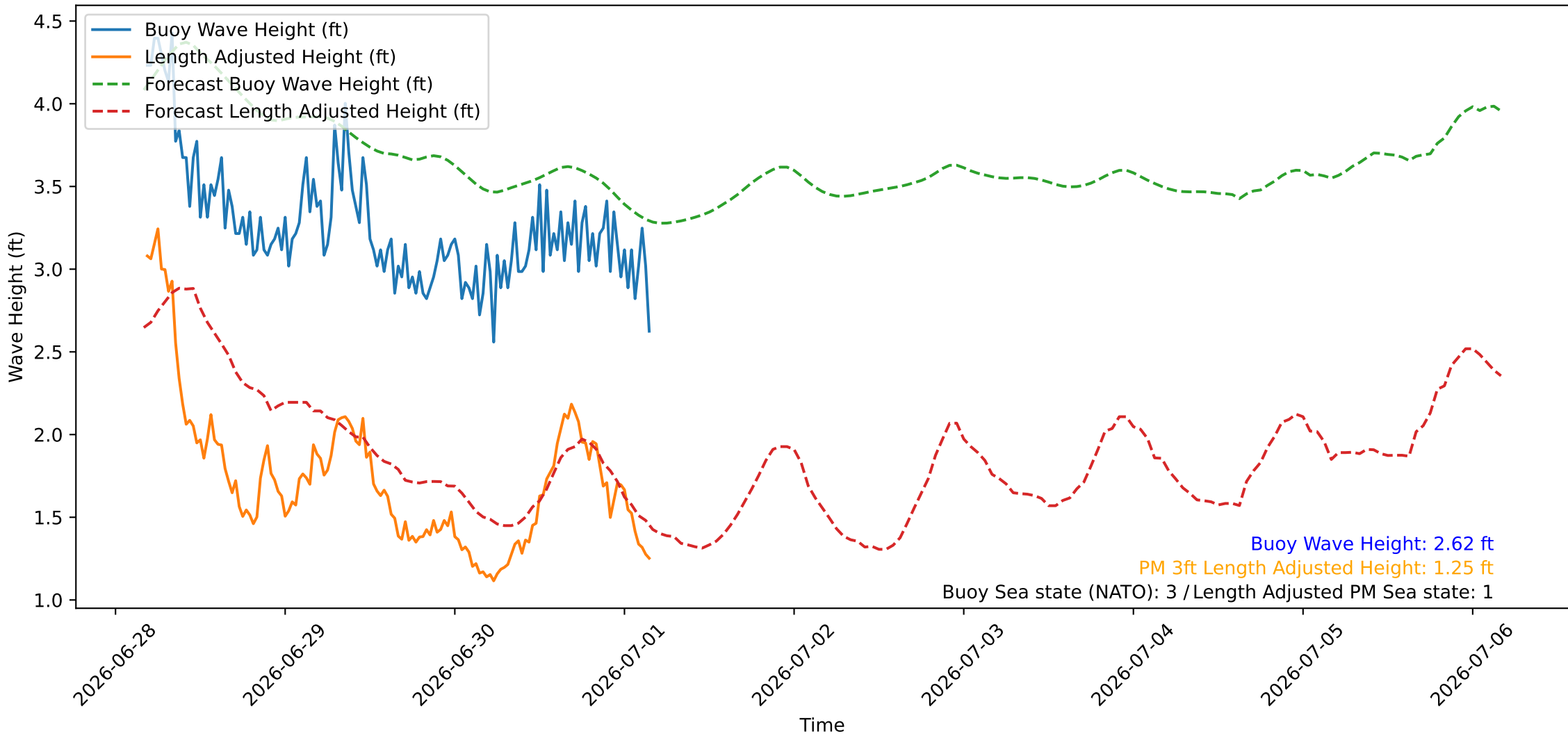
Wave Heights over Time for Oceanside Harbor at 2026-07-01 04:20:25
