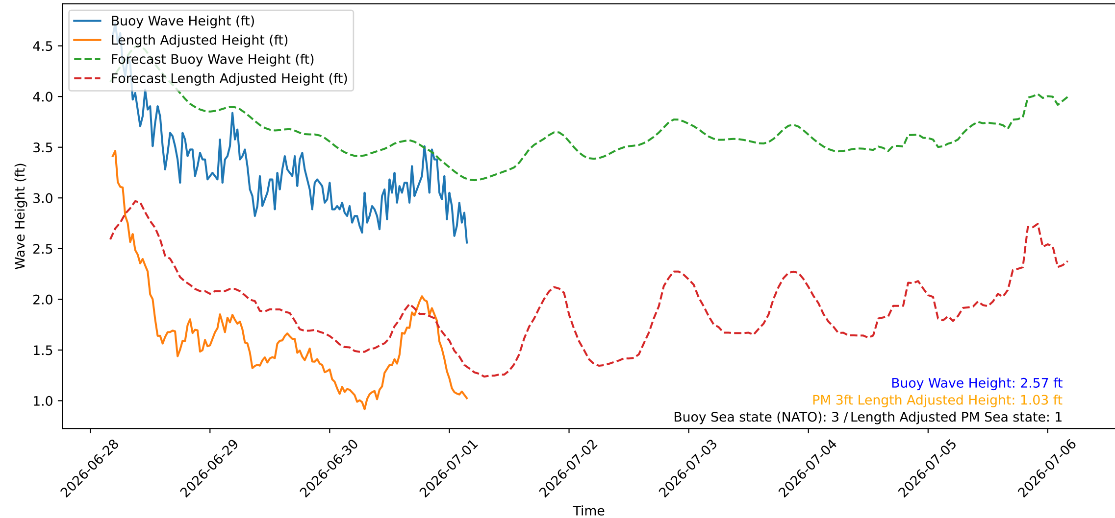
Wave Heights over Time for Green Beach at 2026-07-01 04:21:08
