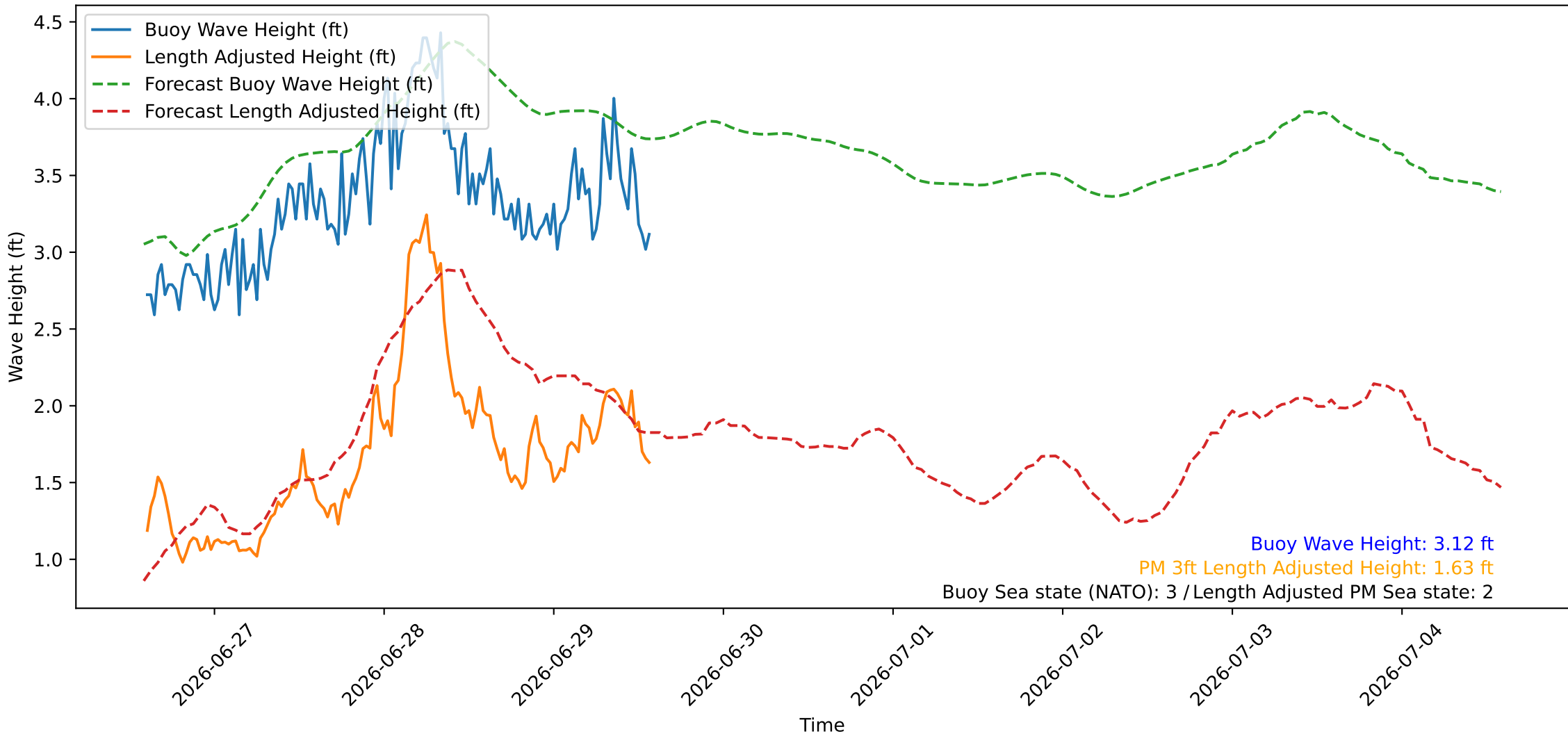
Wave Heights over Time for Oceanside Harbor at 2026-06-29 14:20:26
