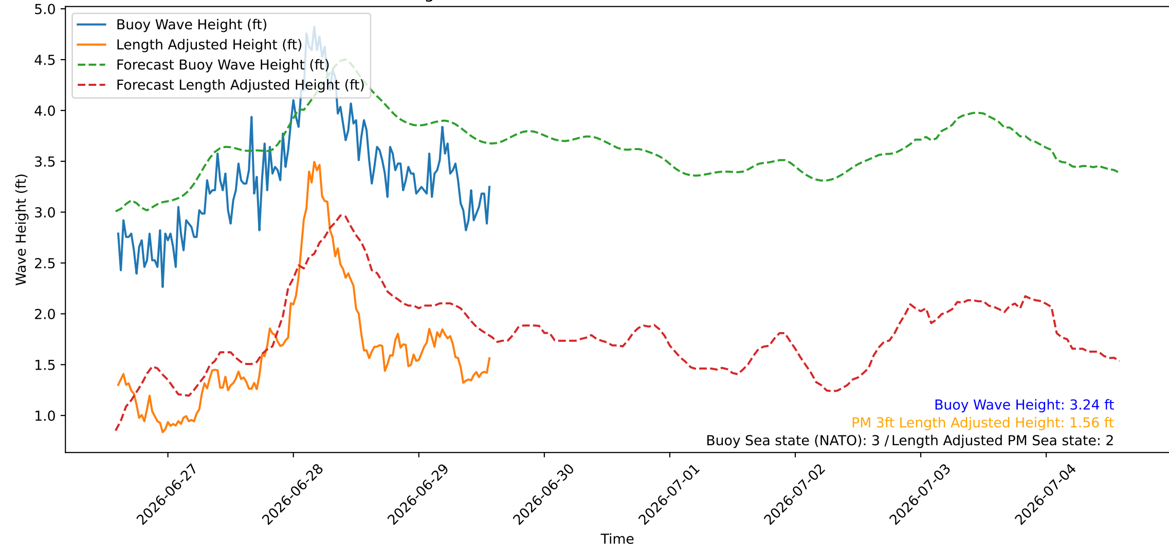
Wave Heights over Time for Green Beach at 2026-06-29 14:21:09
