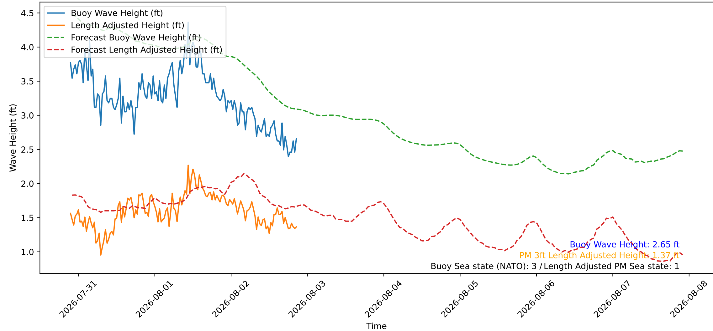
Wave Heights over Time for Oceanside Harbor at 2026-08-02 21:30:26
