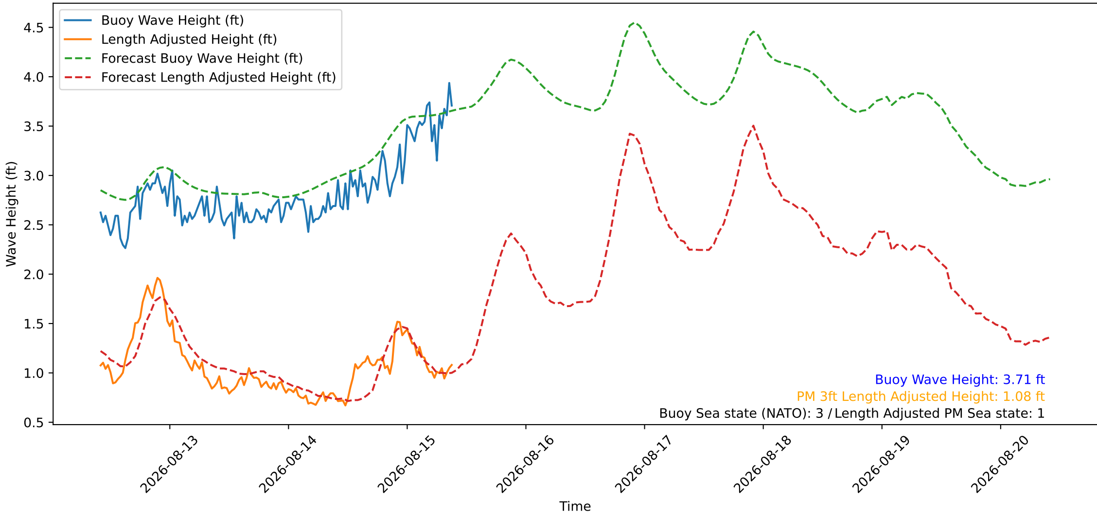
Wave Heights over Time for Green Beach at 2026-08-15 10:01:08
