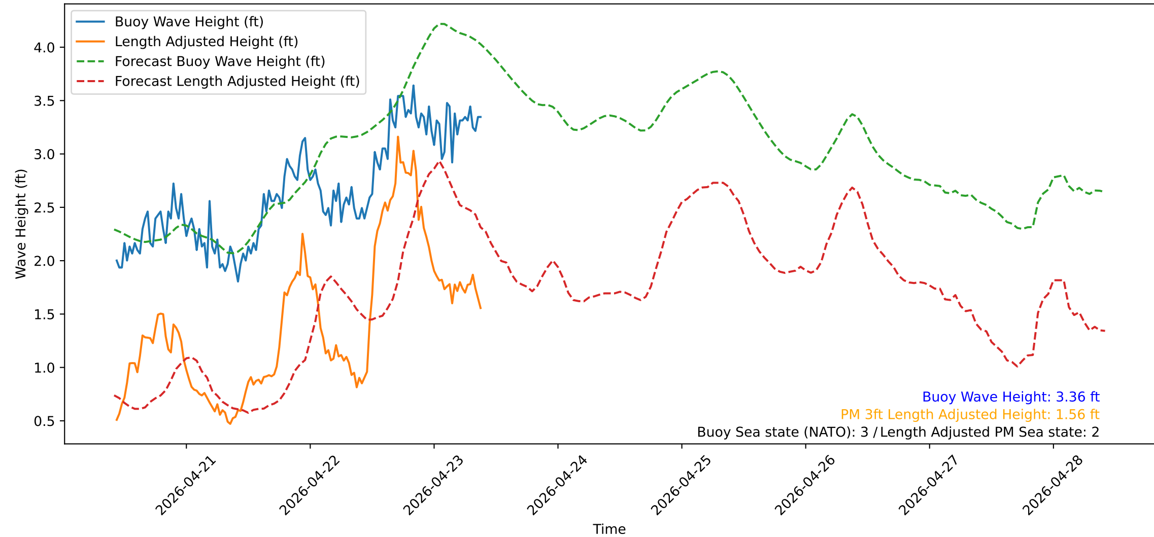
Wave Heights over Time for Red Beach at 2026-04-23 10:00:50
