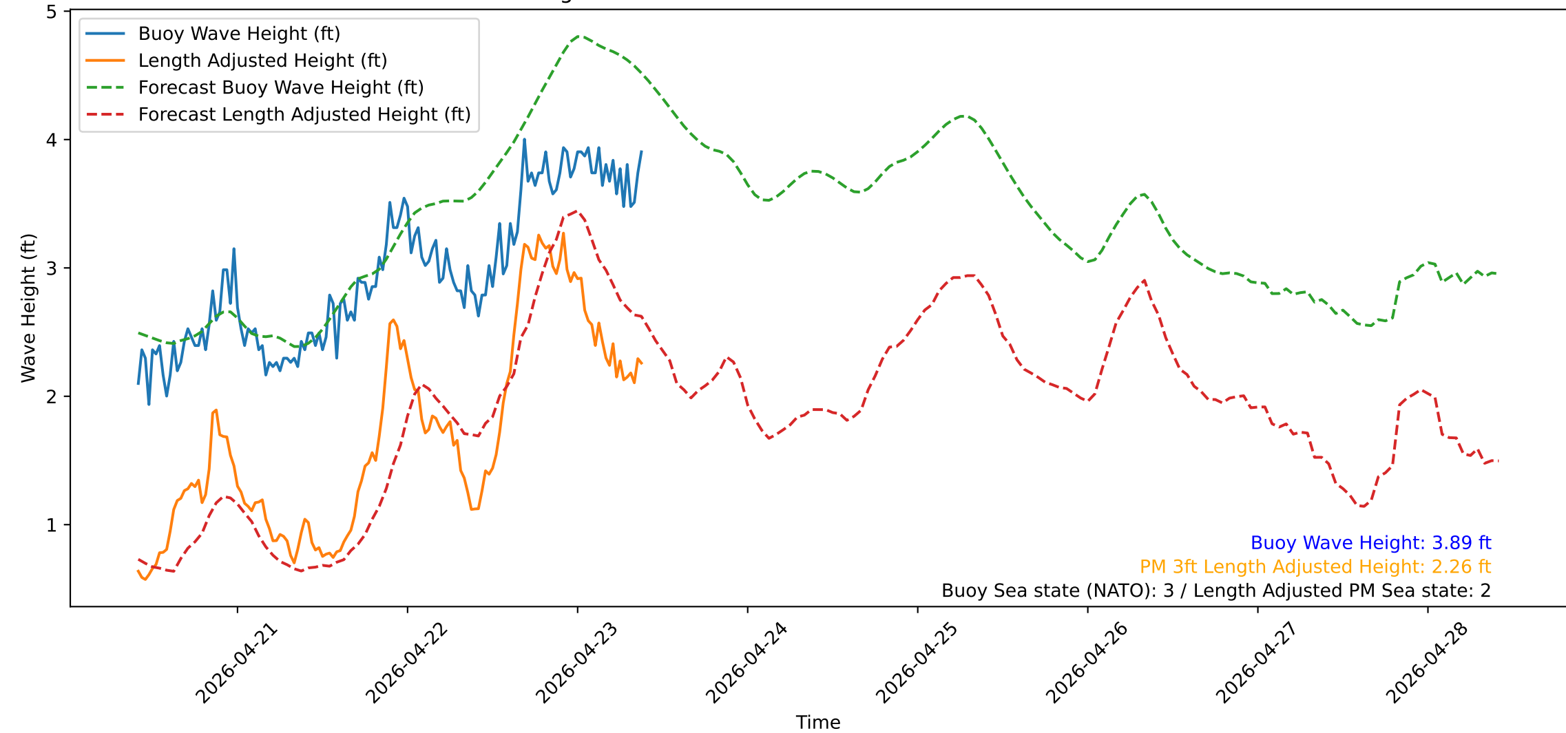
Wave Heights over Time for Green Beach at 2026-04-23 10:01:12
