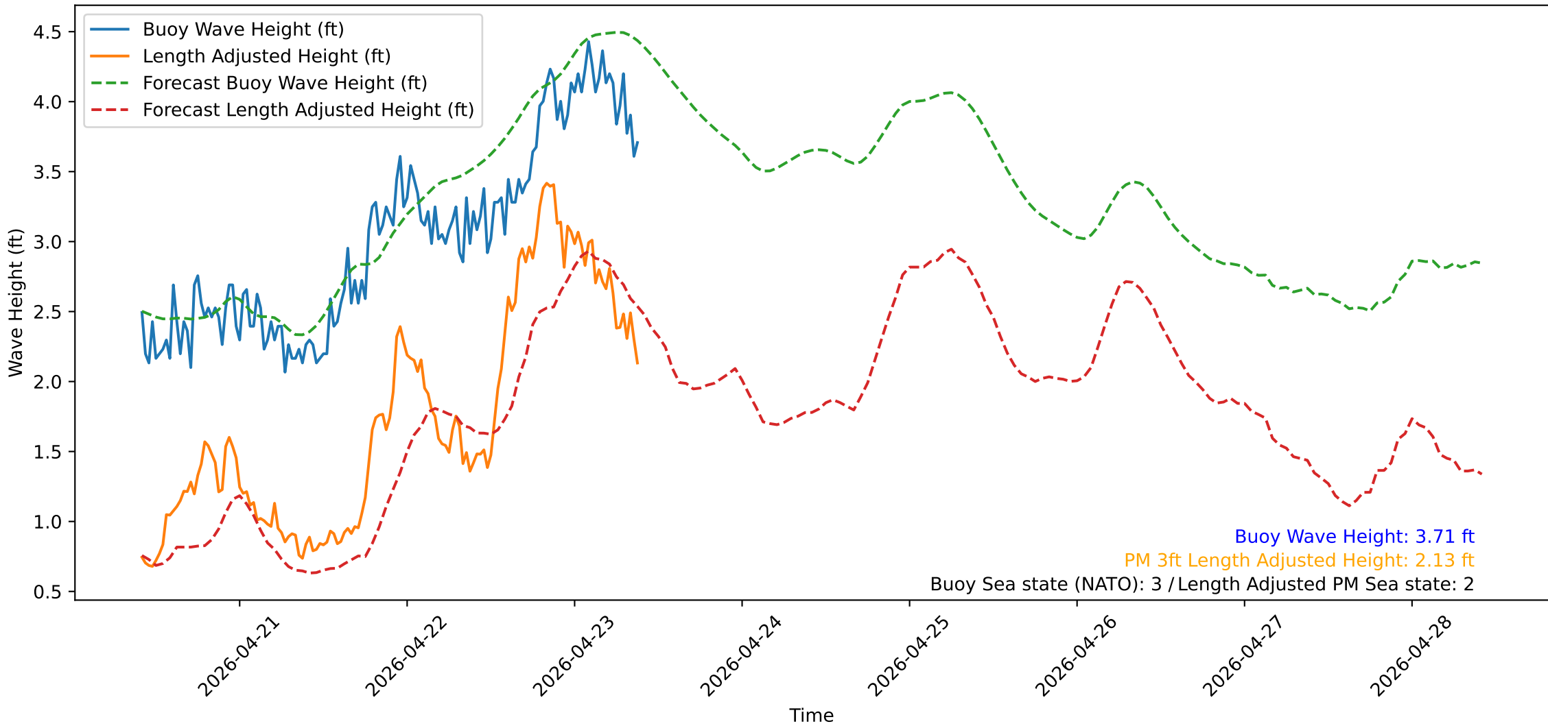
Wave Heights over Time for Oceanside Harbor at 2026-04-23 10:00:31
