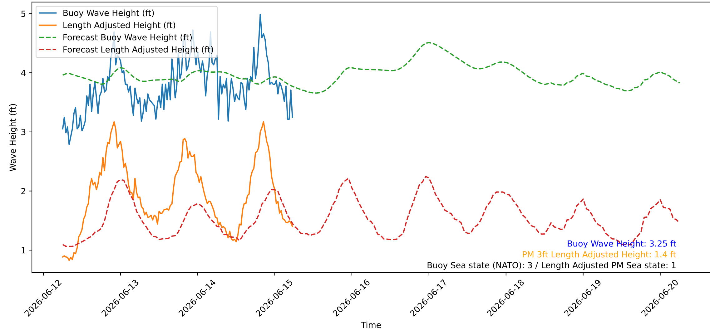
Wave Heights over Time for Oceanside Harbor at 2026-06-15 06:10:26
