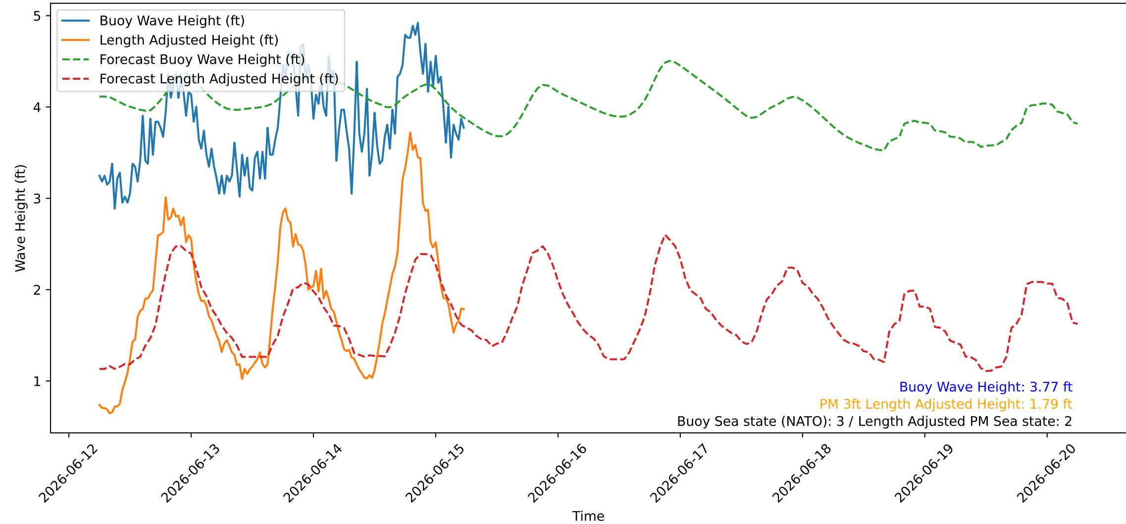
Wave Heights over Time for Green Beach at 2026-06-15 06:11:08
