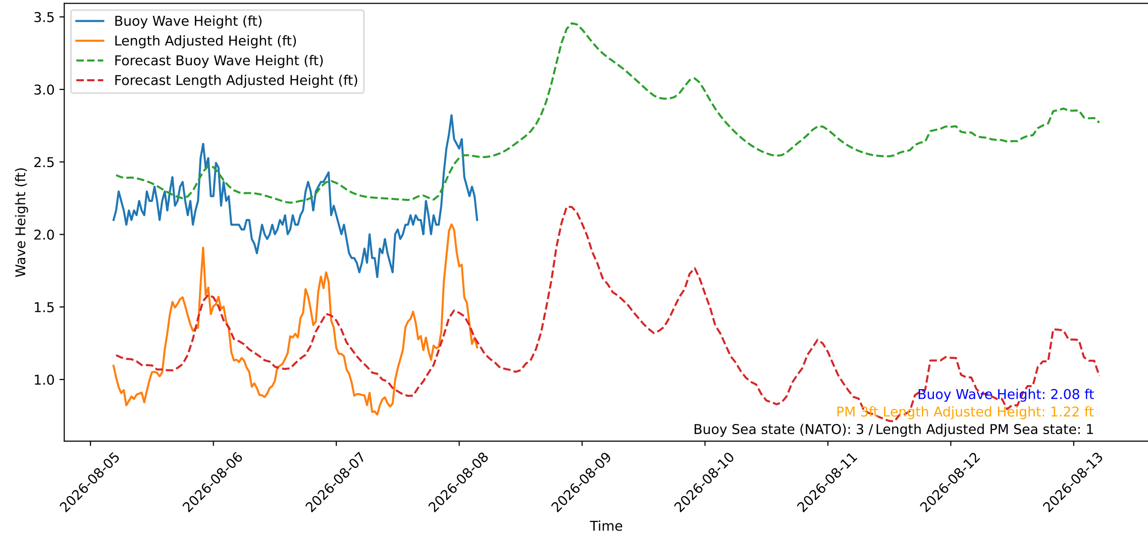
Wave Heights over Time for Green Beach at 2026-08-08 04:31:08
