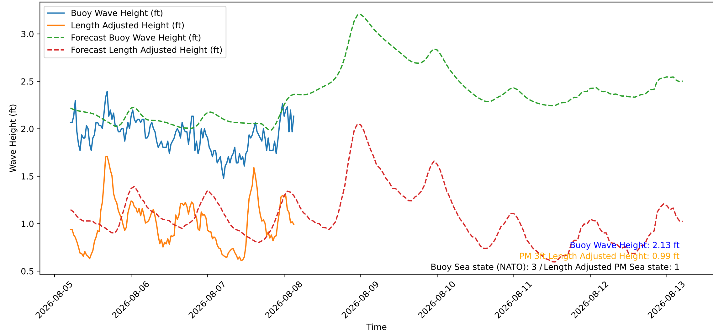
Wave Heights over Time for Red Beach at 2026-08-08 04:30:45
