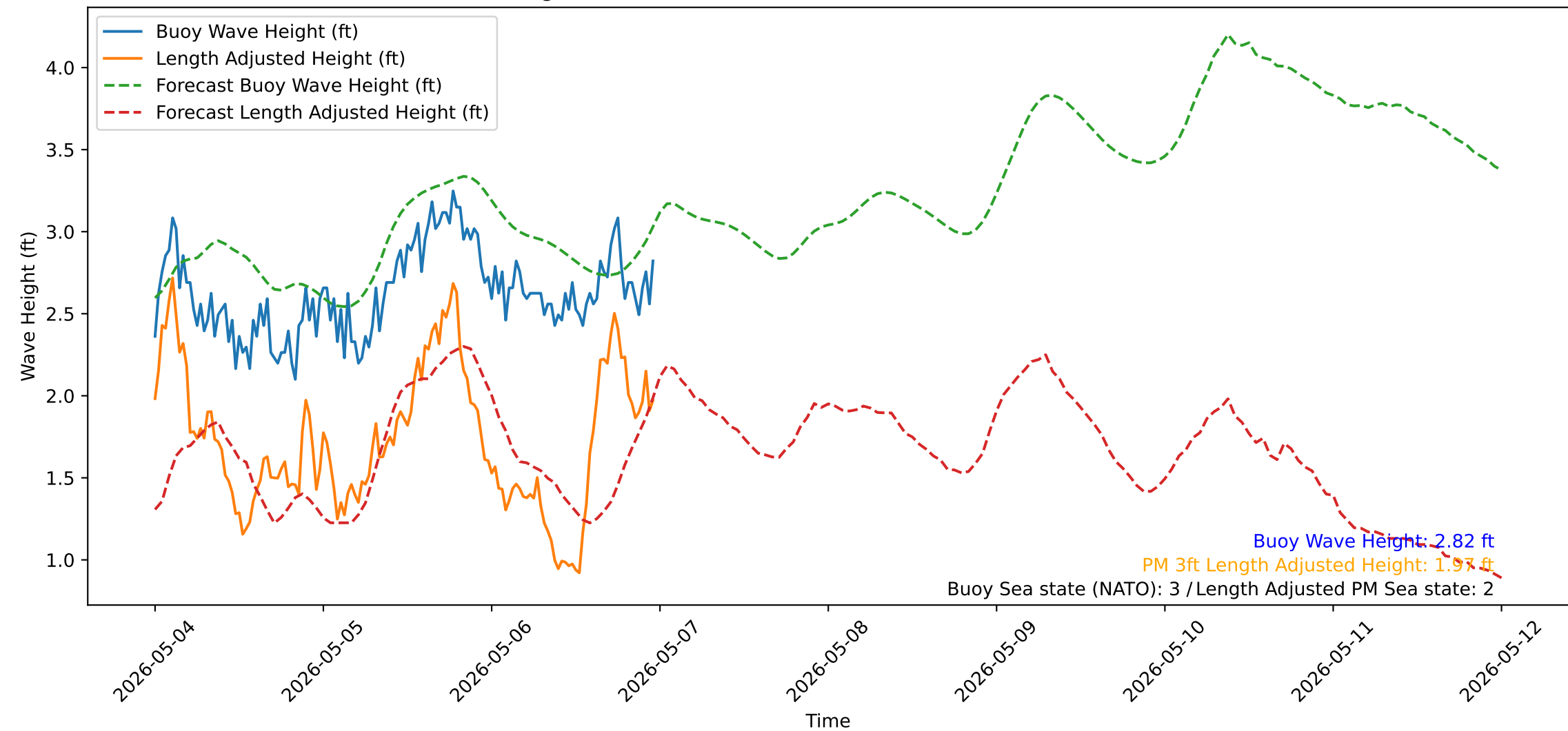
Wave Heights over Time for Oceanside Harbor at 2026-05-06 23:50:32
