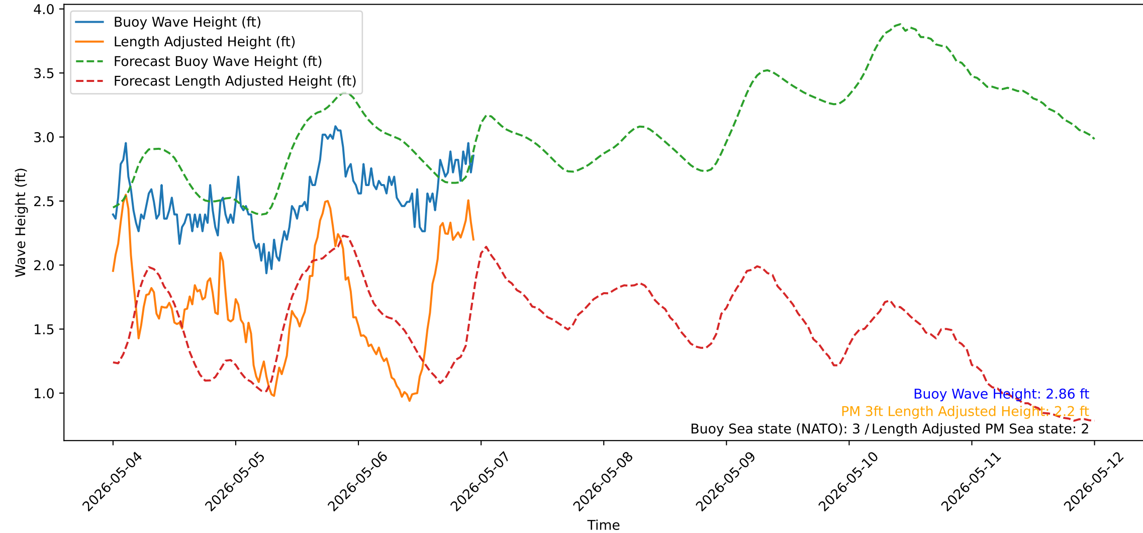
Wave Heights over Time for Red Beach at 2026-05-06 23:50:52
