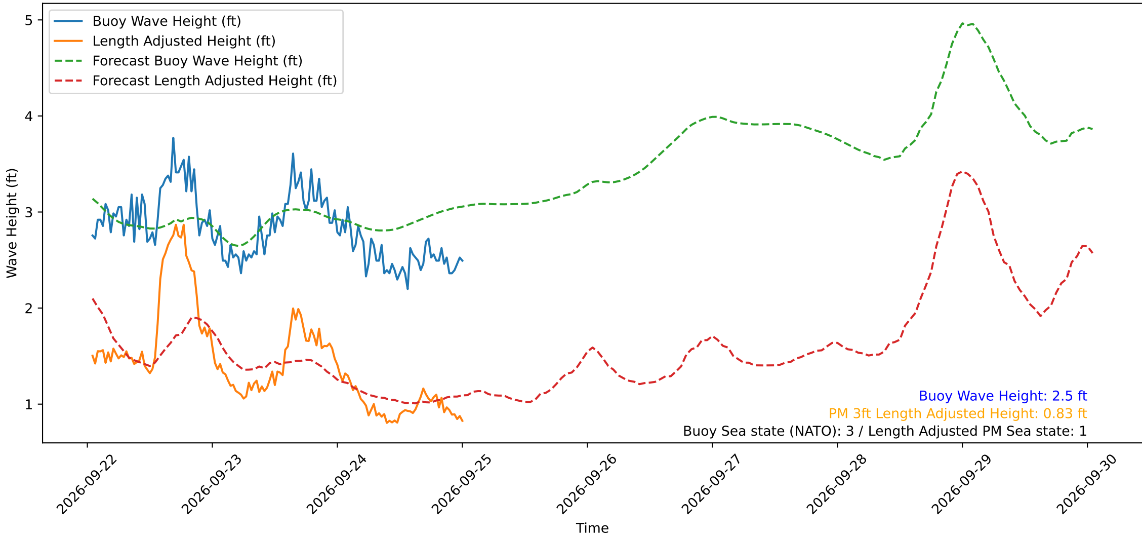
Wave Heights over Time for Oceanside Harbor at 2026-09-25 01:00:30
