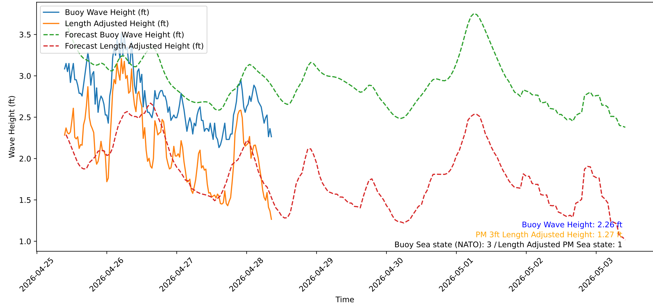
Wave Heights over Time for Green Beach at 2026-04-28 09:31:13
