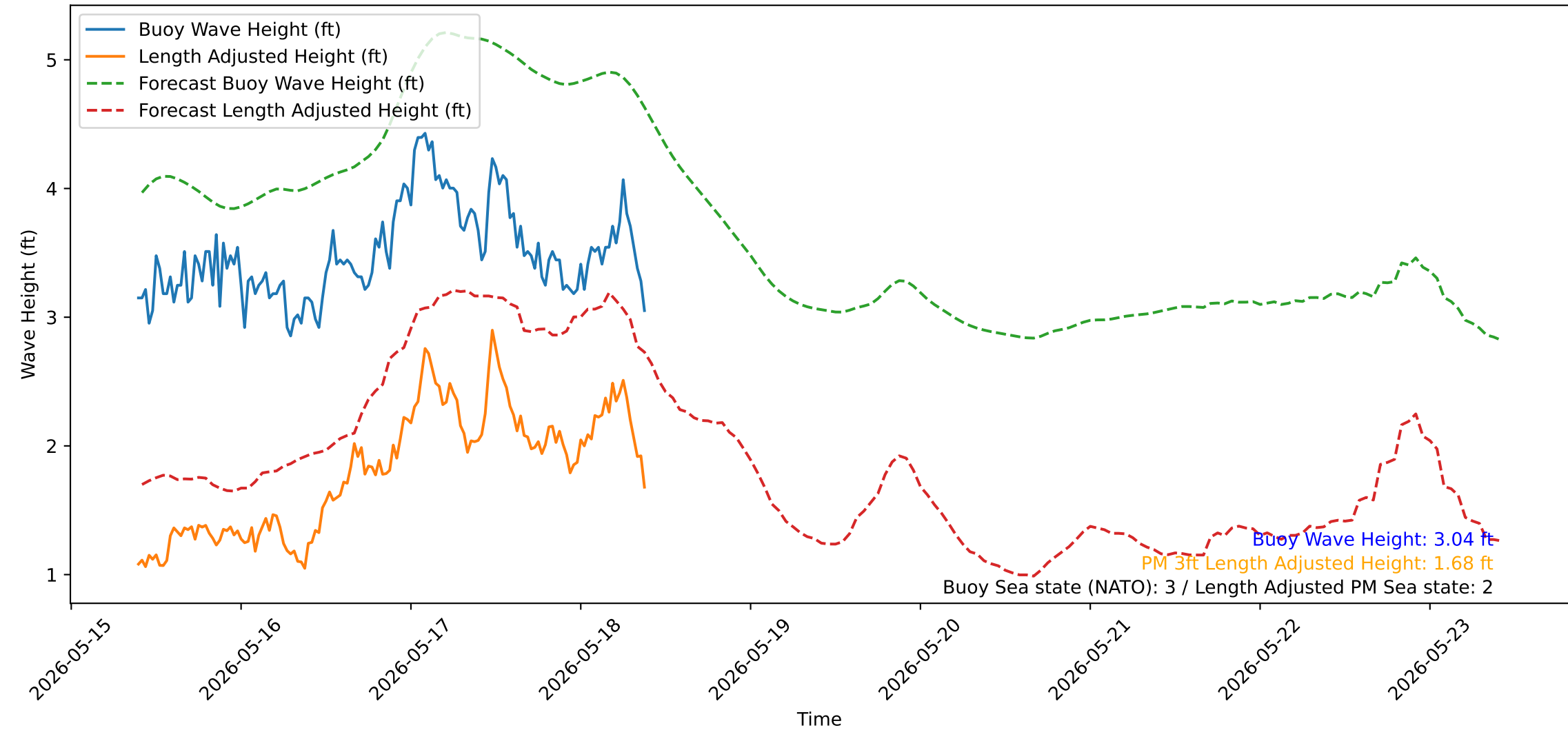
Wave Heights over Time for Green Beach at 2026-05-18 09:41:13
