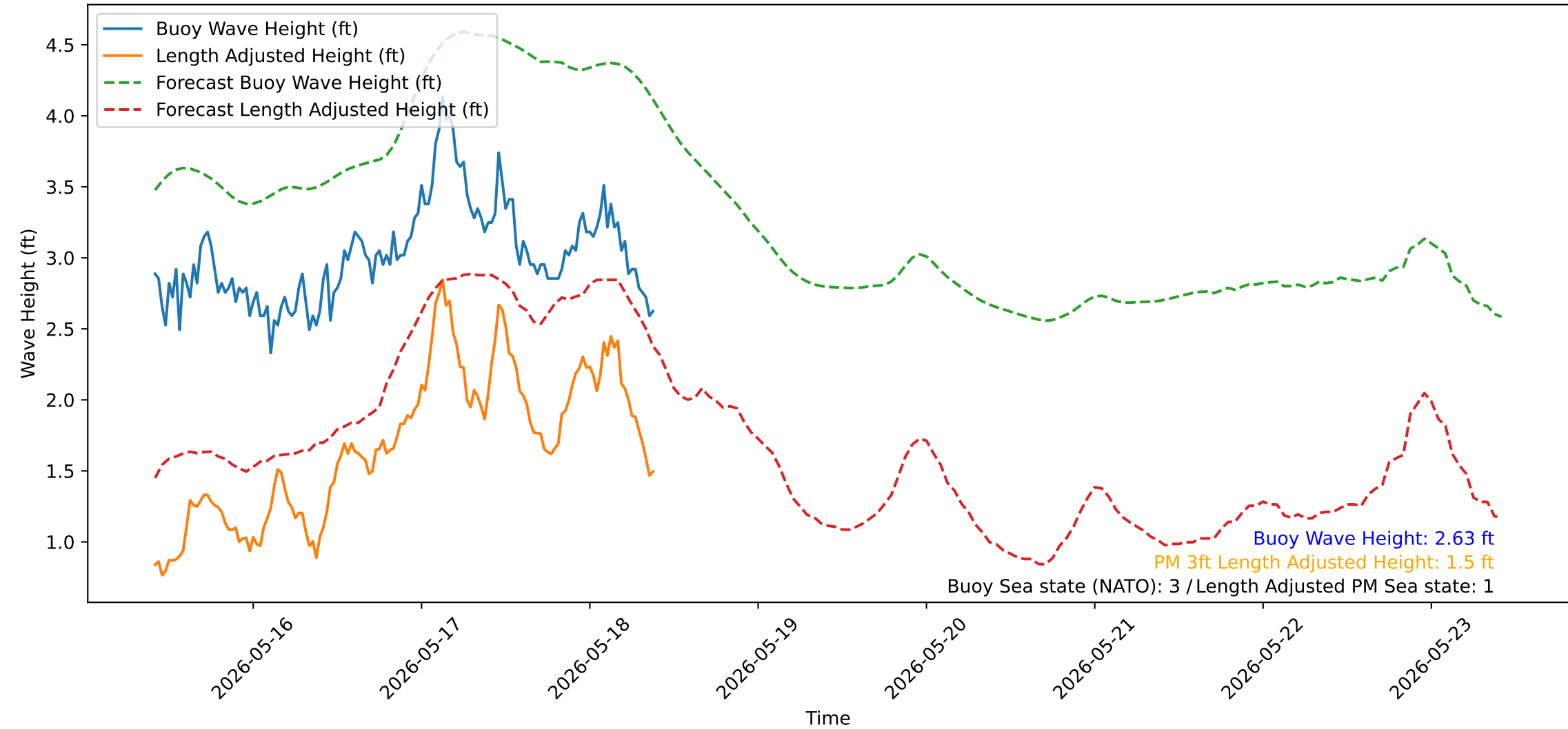
Wave Heights over Time for Red Beach at 2026-05-18 09:40:50
