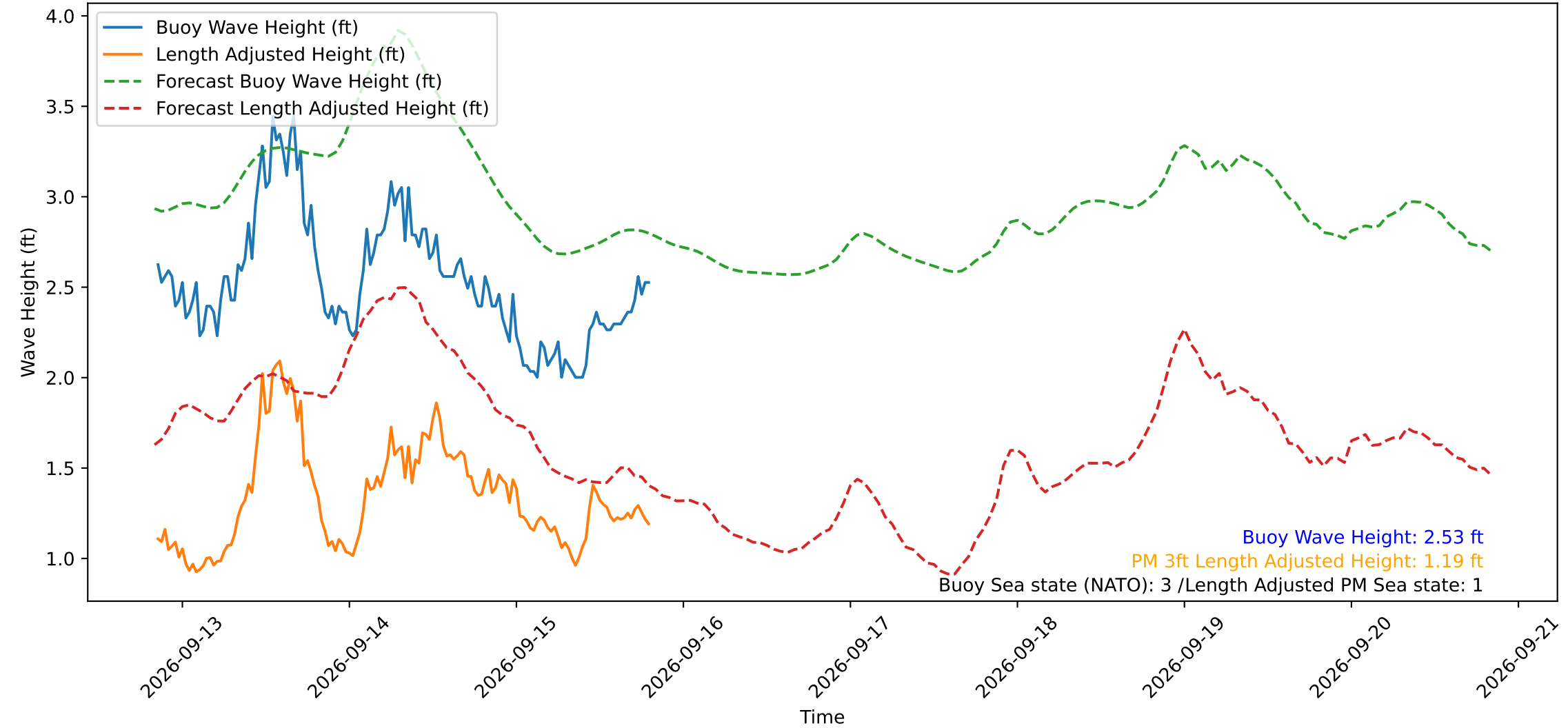
Wave Heights over Time for Red Beach at 2026-09-15 20:00:49
