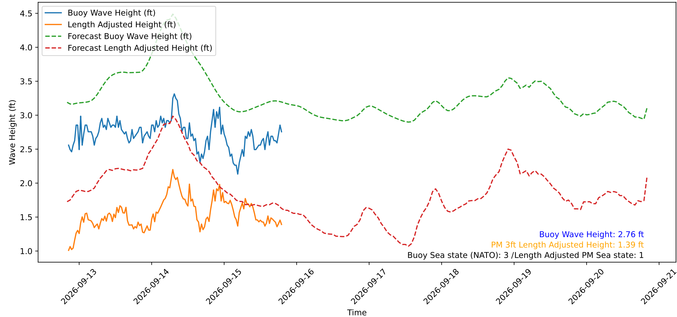
Wave Heights over Time for Green Beach at 2026-09-15 20:01:11
