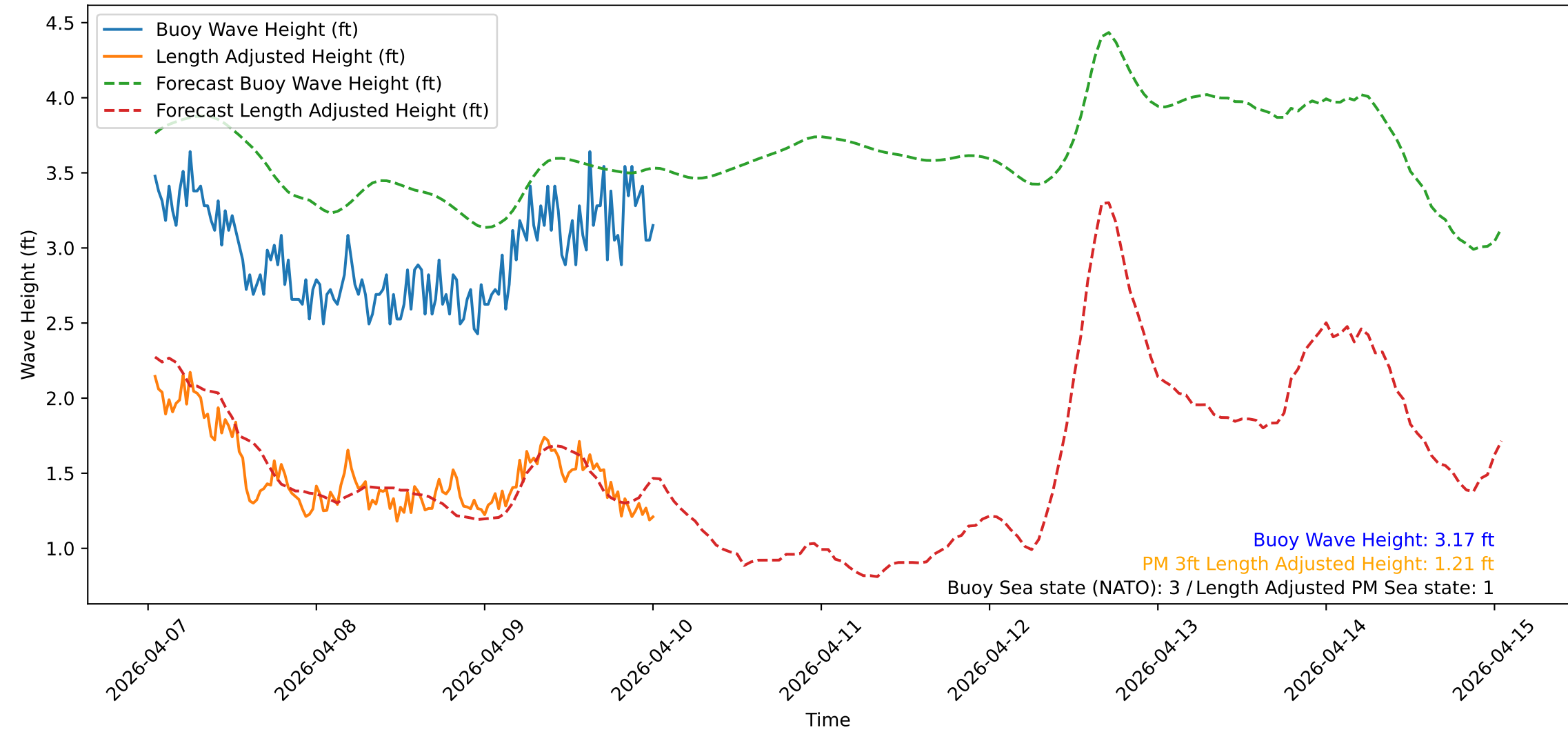
Wave Heights over Time for Oceanside Harbor at 2026-04-10 01:10:31
