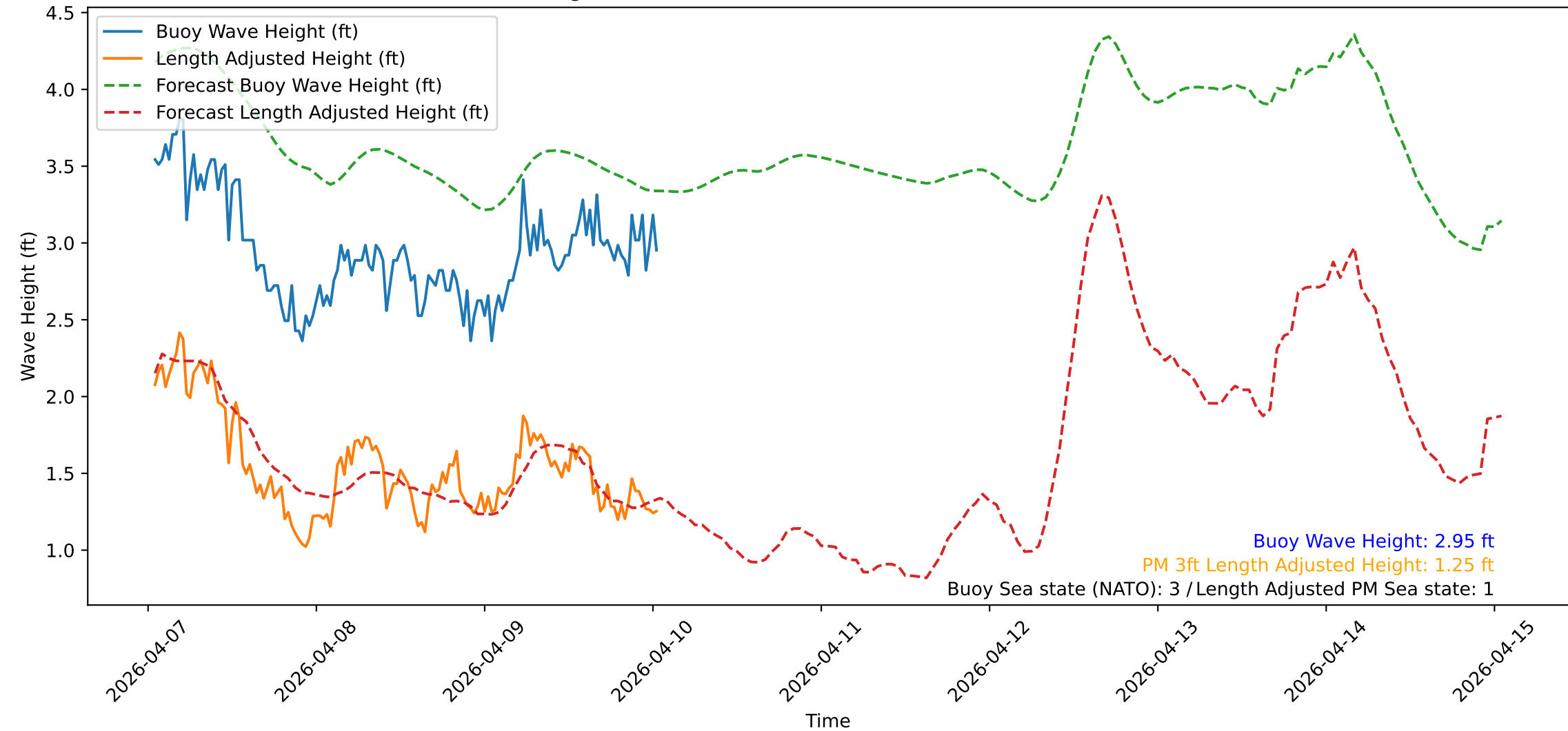
Wave Heights over Time for Green Beach at 2026-04-10 01:11:12
