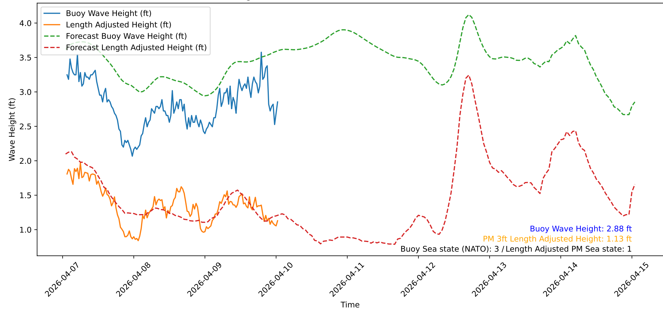
Wave Heights over Time for Red Beach at 2026-04-10 01:10:50
