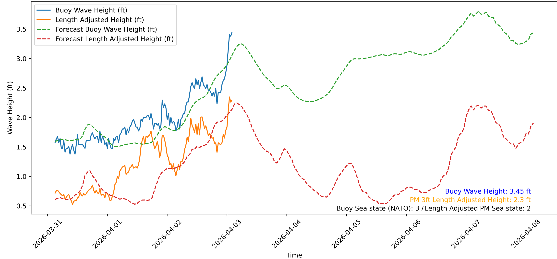
Wave Heights over Time for Red Beach at 2026-04-03 02:50:47
