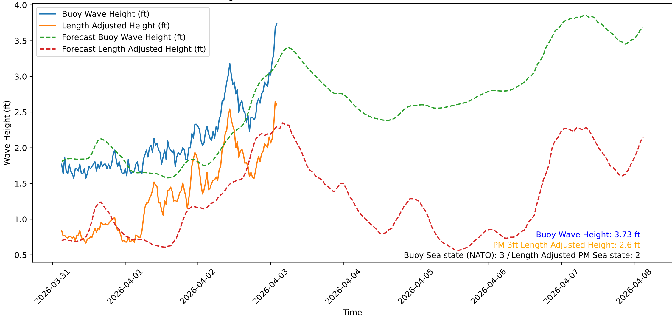
Wave Heights over Time for Oceanside Harbor at 2026-04-03 02:50:31
