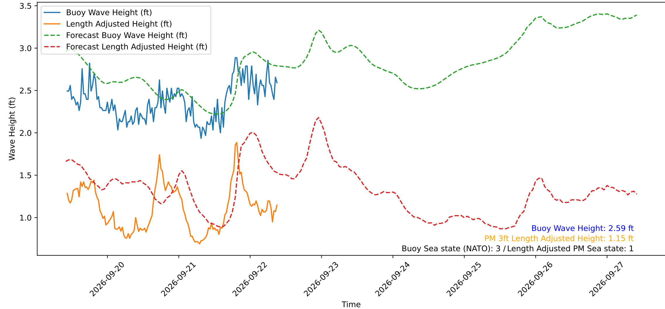
Wave Heights over Time for Red Beach at 2026-09-22 10:00:49
