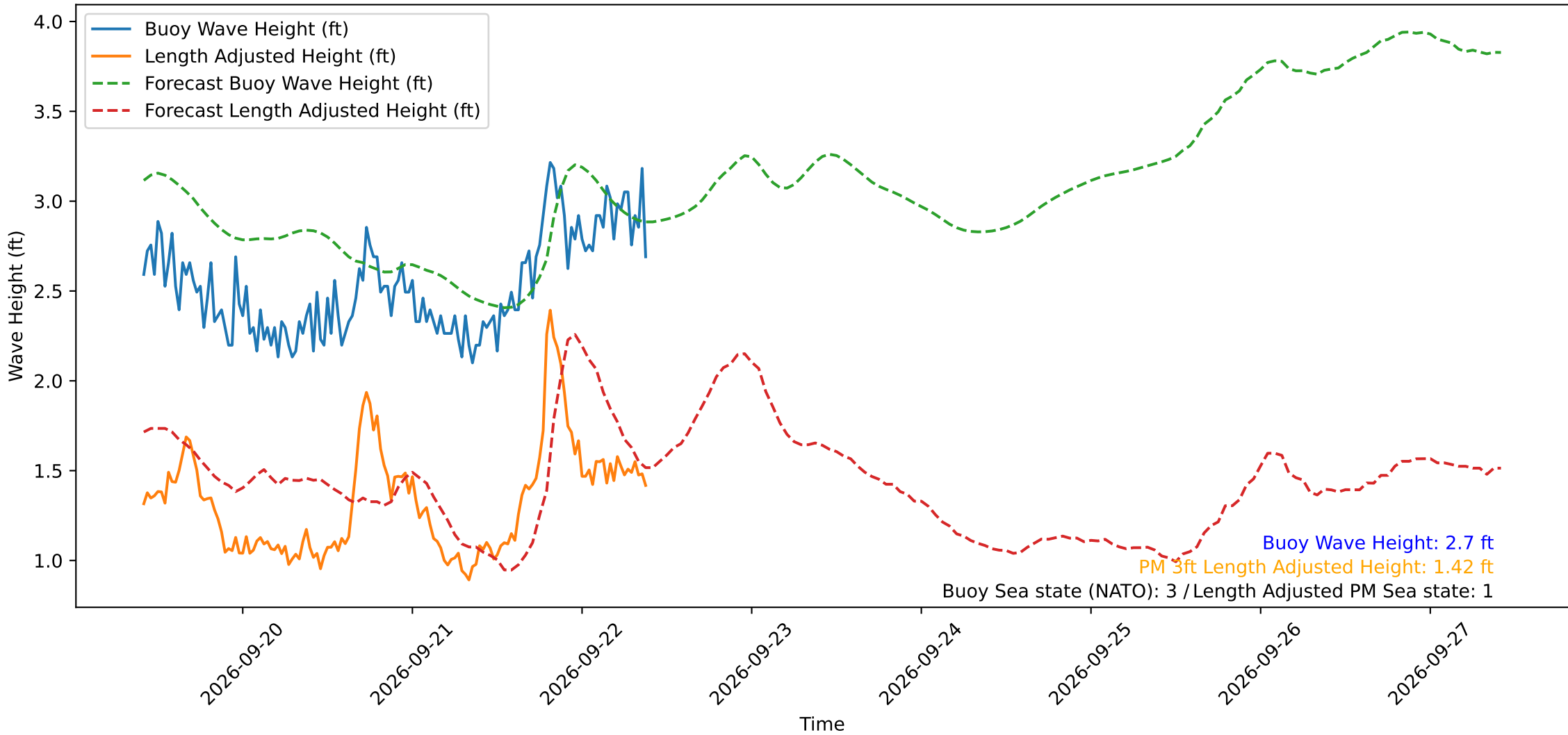
Wave Heights over Time for Oceanside Harbor at 2026-09-22 10:00:29
