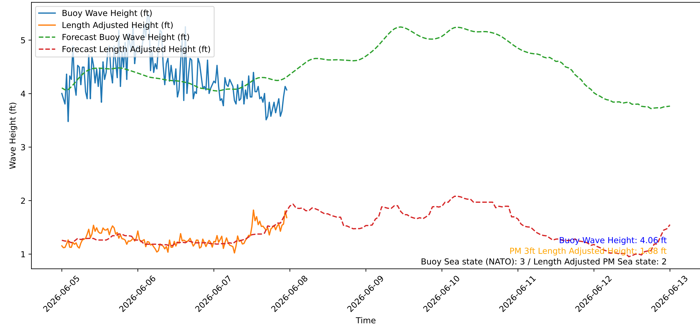
Wave Heights over Time for Oceanside Harbor at 2026-06-07 23:50:26
