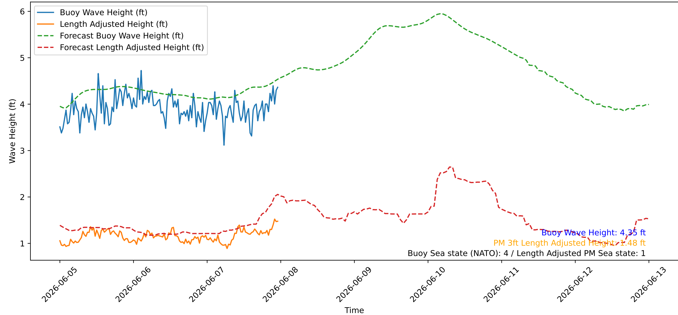
Wave Heights over Time for Green Beach at 2026-06-07 23:51:09
