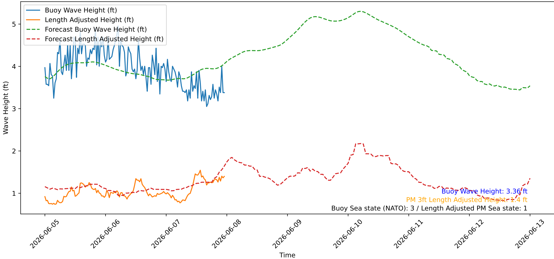
Wave Heights over Time for Red Beach at 2026-06-07 23:50:47
