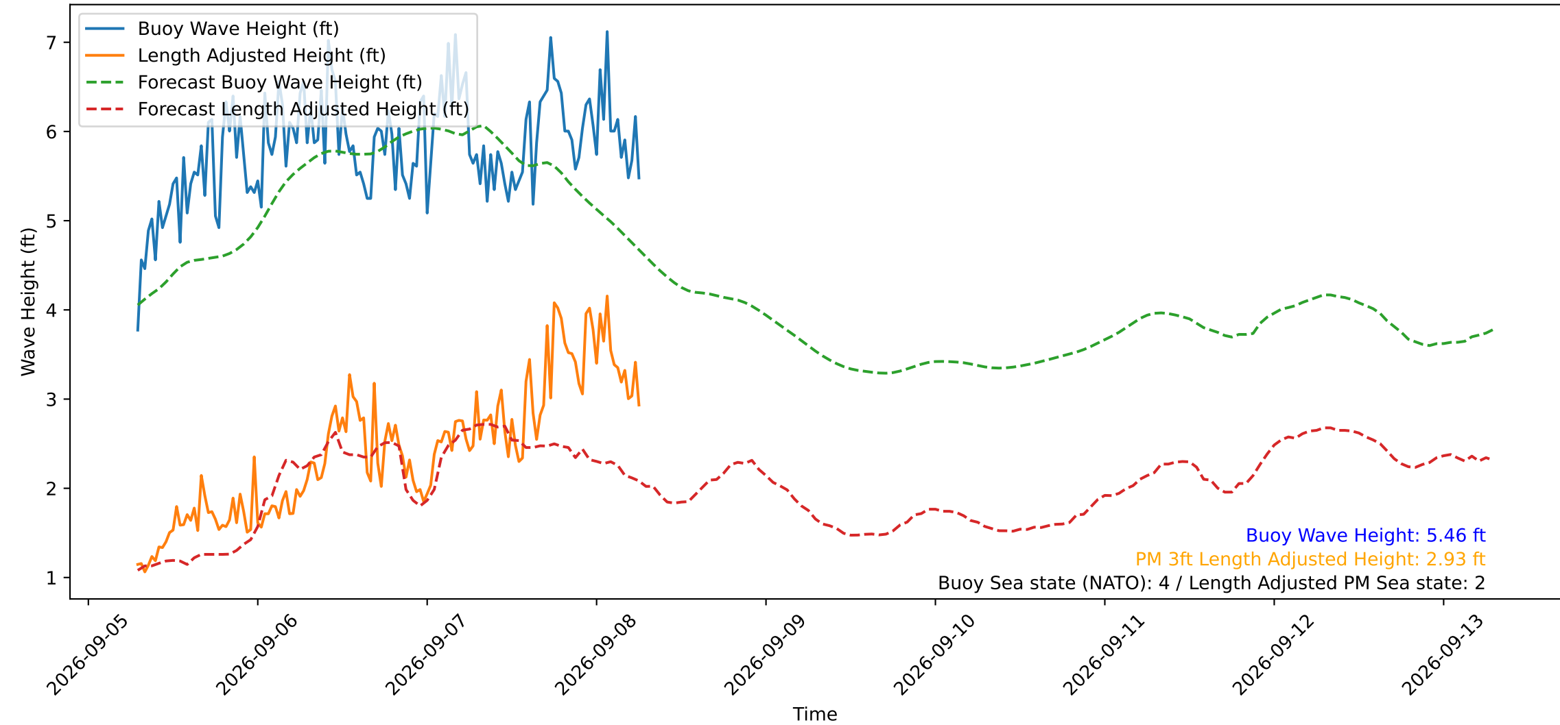
Wave Heights over Time for Oceanside Harbor at 2026-09-08 06:50:30
