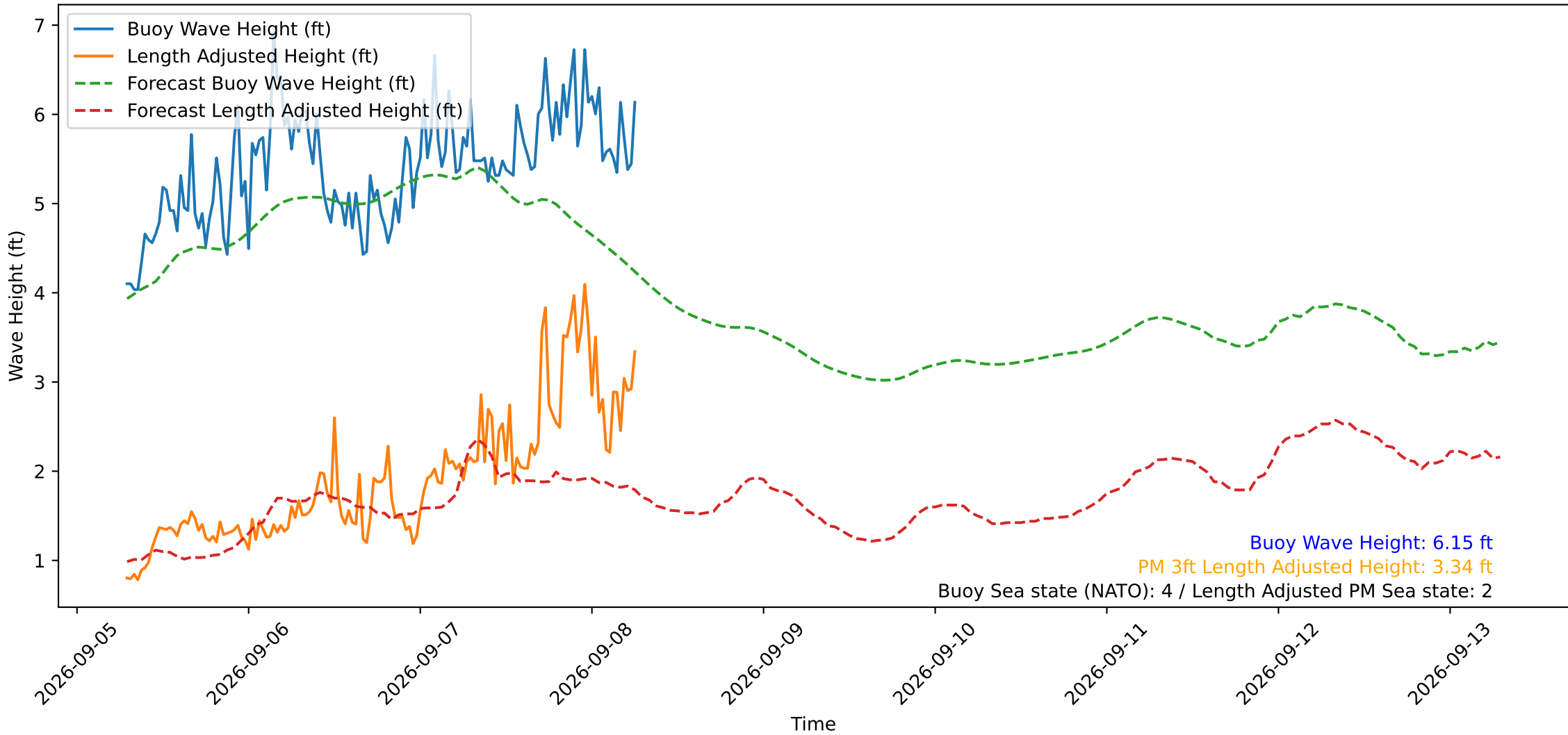
Wave Heights over Time for Red Beach at 2026-09-08 06:50:51
