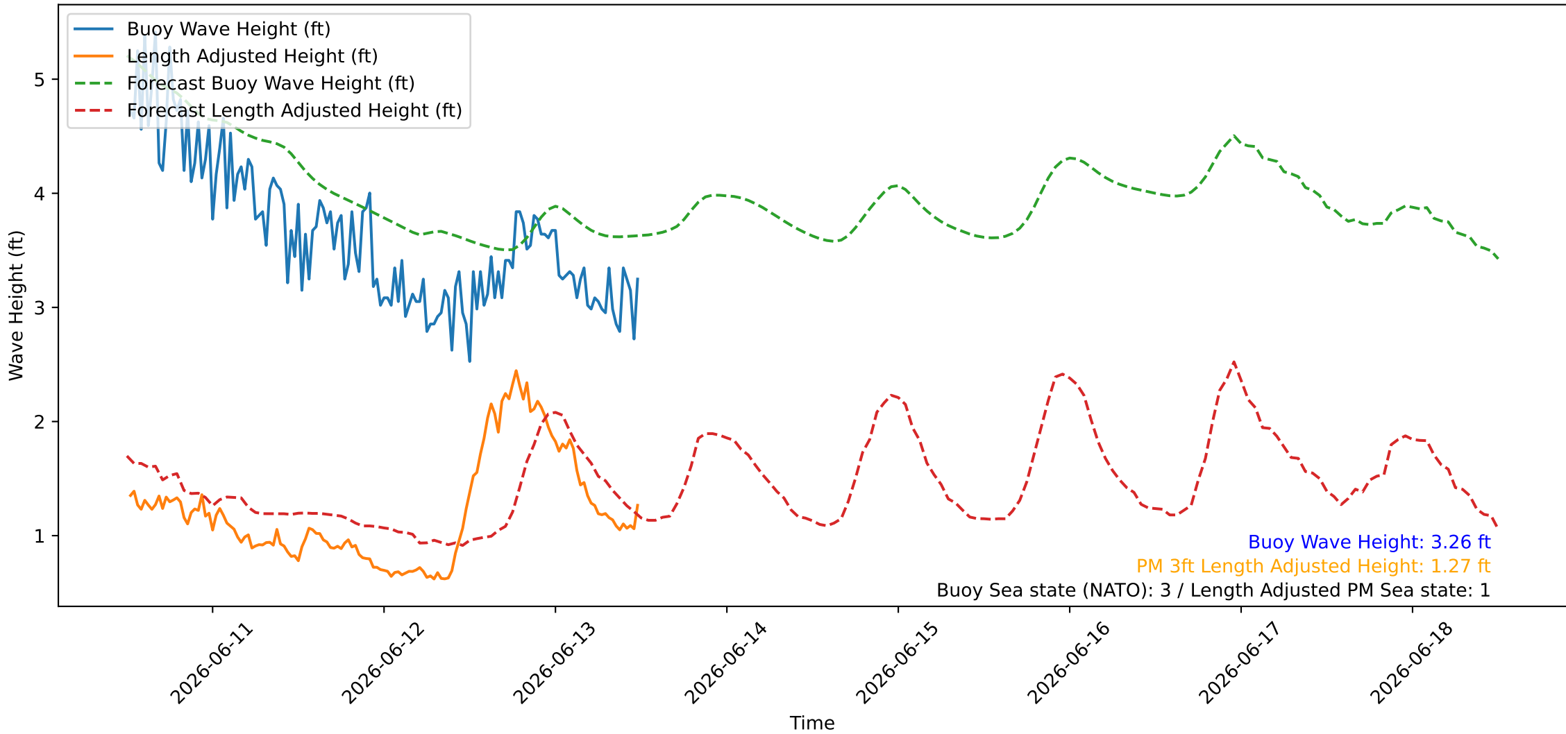
Wave Heights over Time for Red Beach at 2026-06-13 12:20:47
