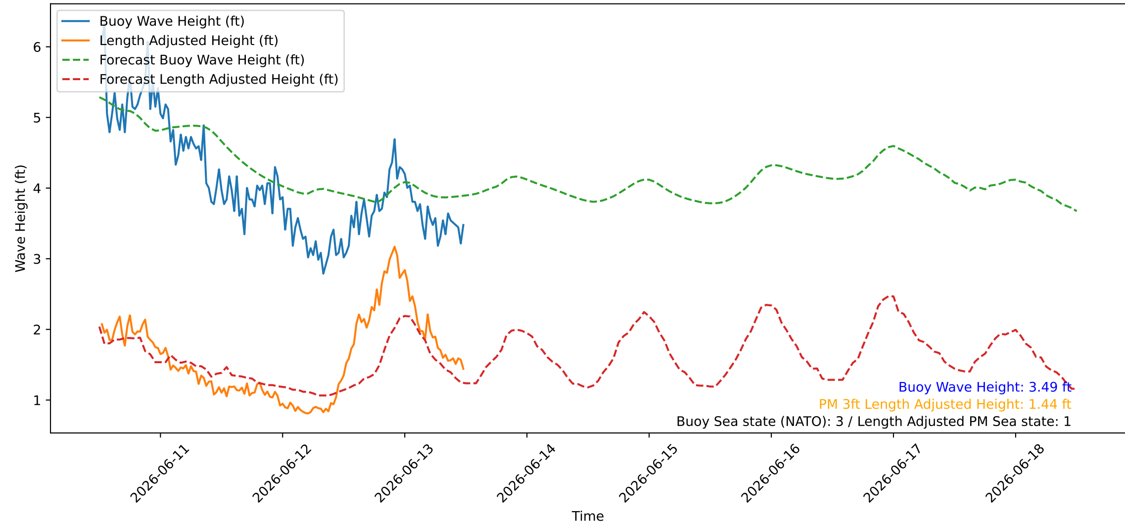
Wave Heights over Time for Oceanside Harbor at 2026-06-13 12:20:27
