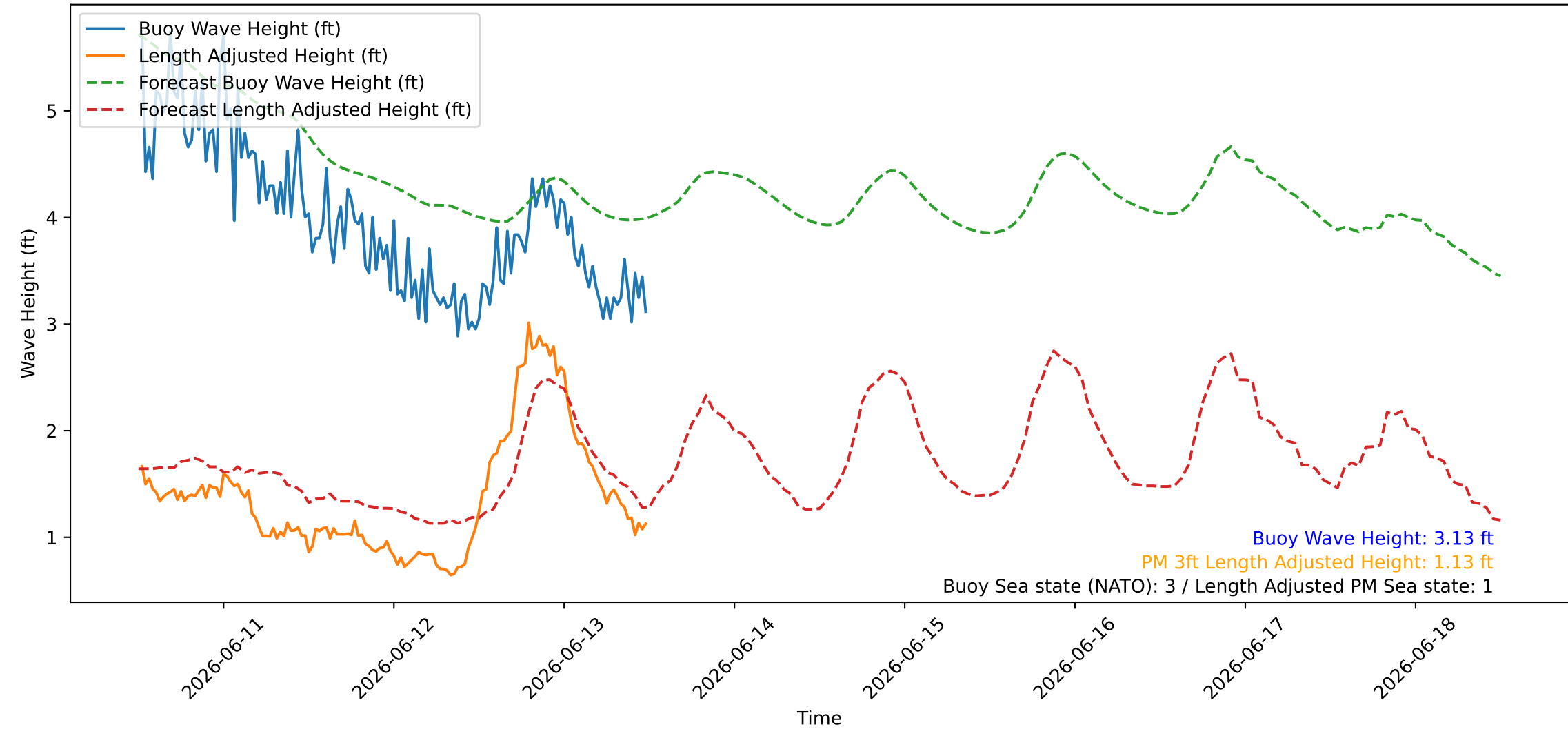
Wave Heights over Time for Green Beach at 2026-06-13 12:21:11
