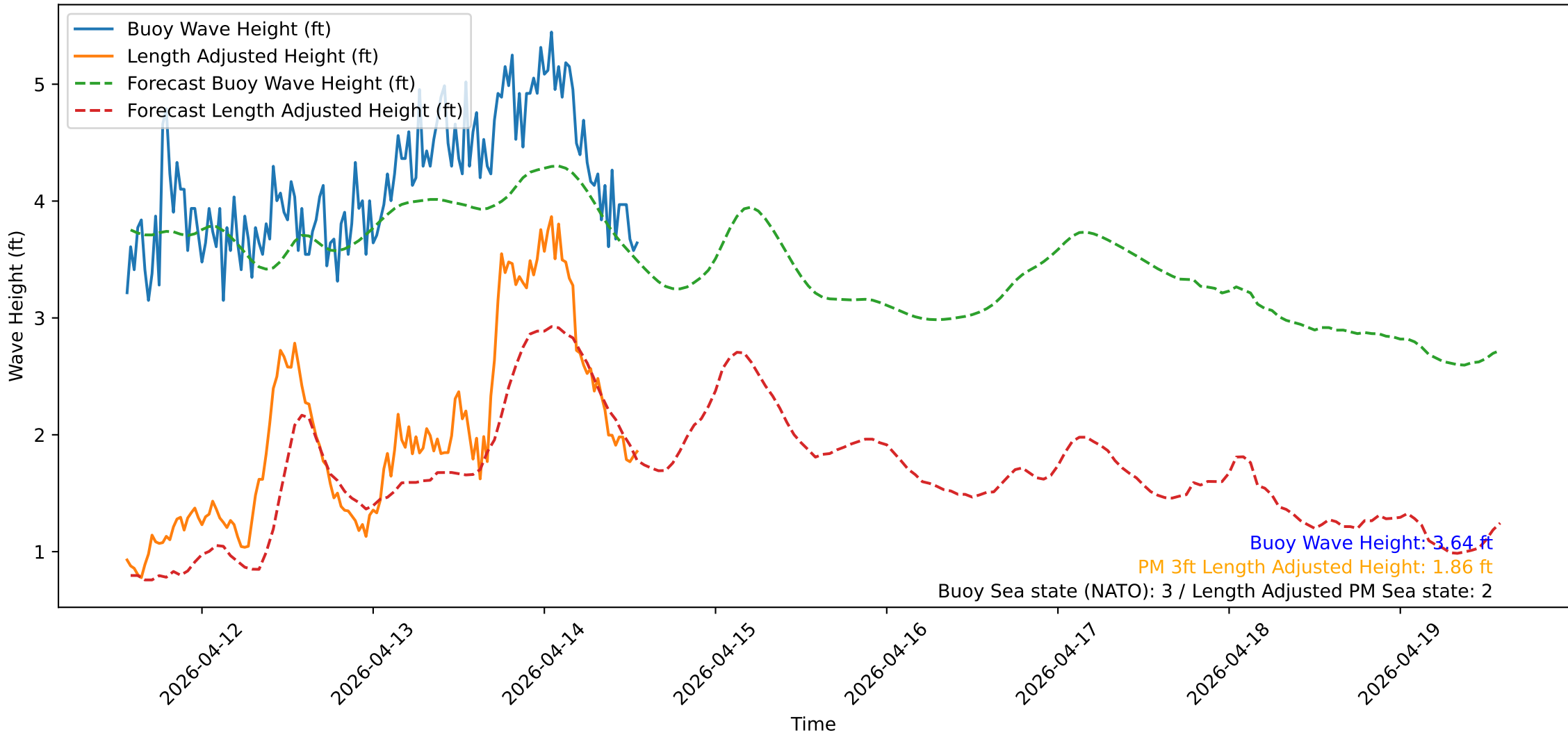
Wave Heights over Time for Oceanside Harbor at 2026-04-14 13:30:32
