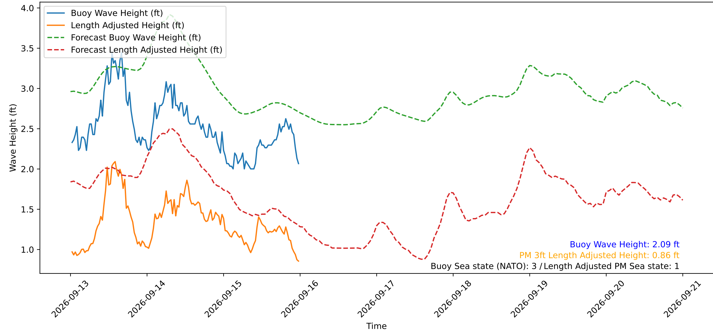
Wave Heights over Time for Red Beach at 2026-09-16 00:10:49
