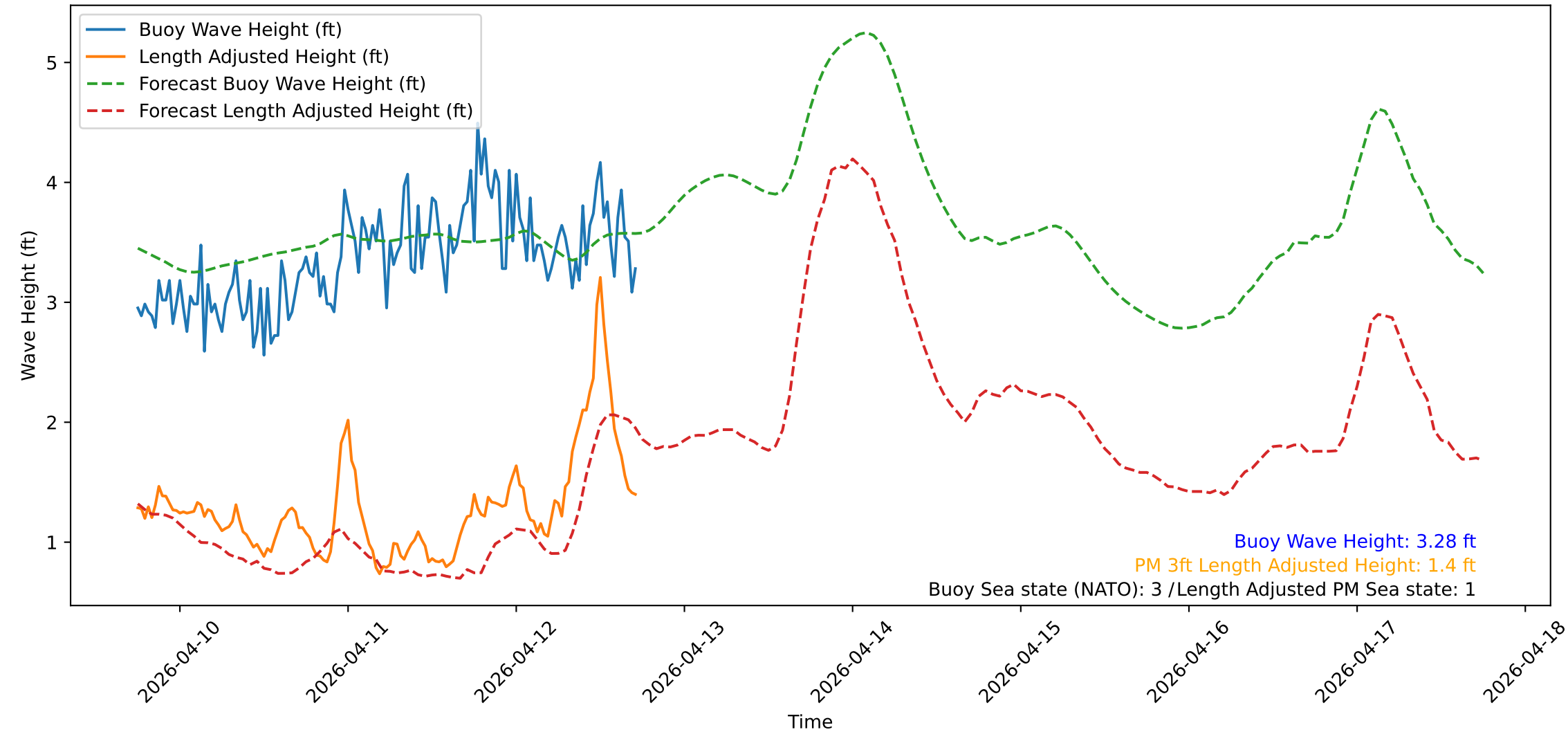
Wave Heights over Time for Green Beach at 2026-04-12 17:51:12
