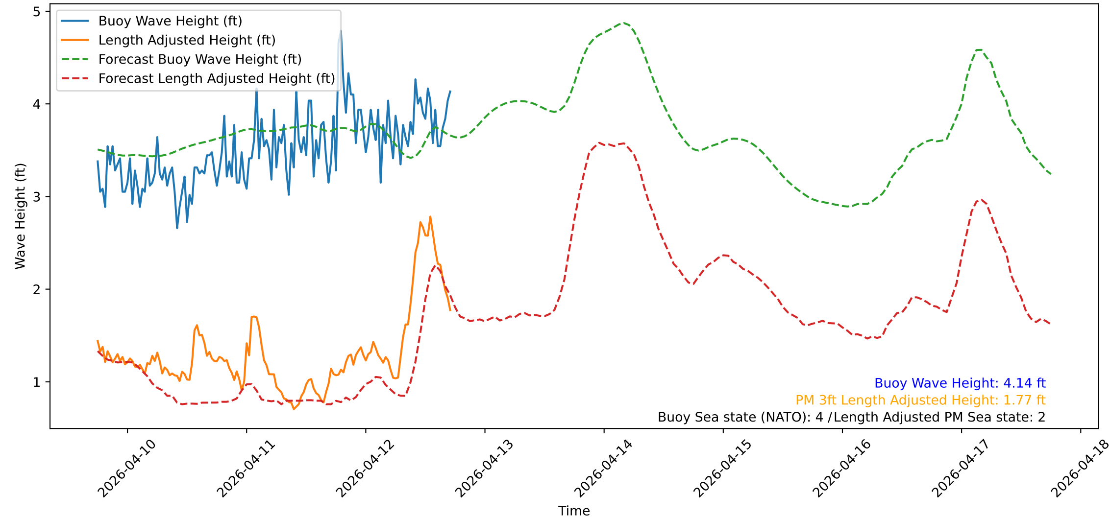
Wave Heights over Time for Oceanside Harbor at 2026-04-12 17:50:30
