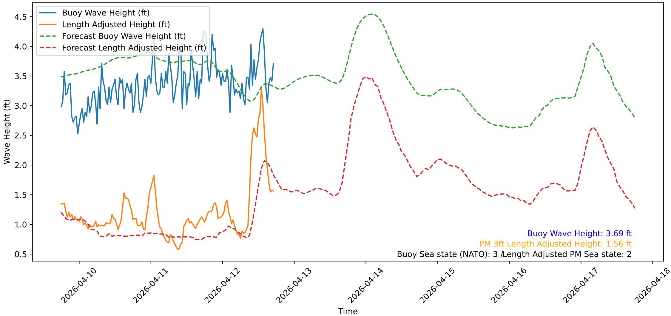
Wave Heights over Time for Red Beach at 2026-04-12 17:50:50
