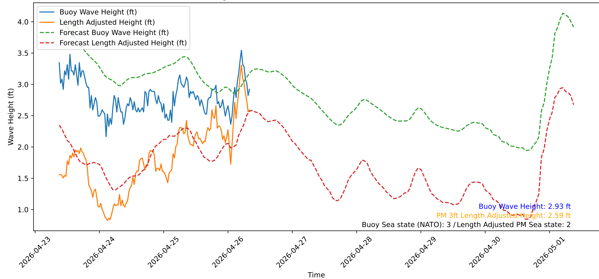
Wave Heights over Time for Red Beach at 2026-04-26 08:40:50
