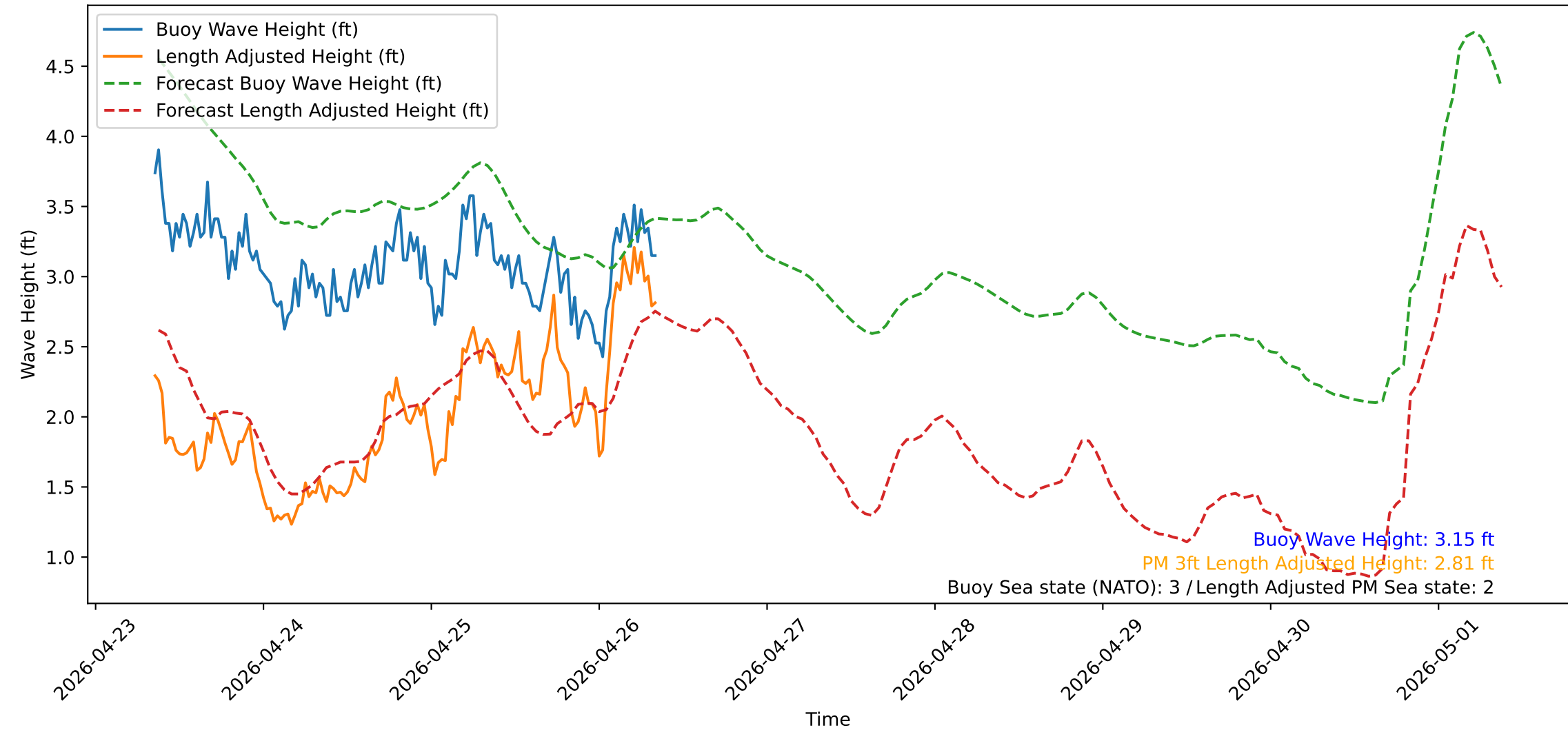
Wave Heights over Time for Green Beach at 2026-04-26 08:41:12
