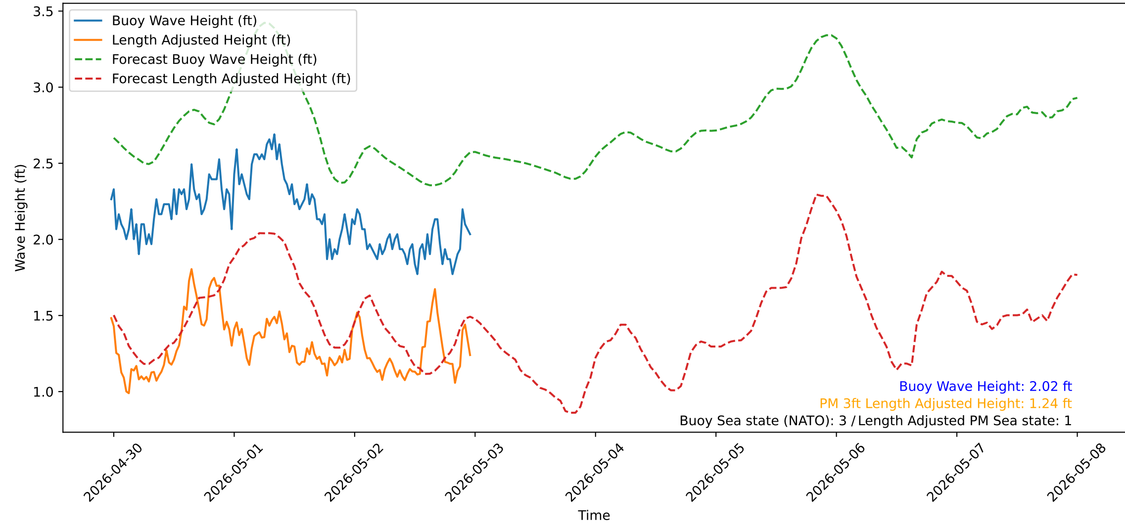
Wave Heights over Time for Oceanside Harbor at 2026-05-02 23:40:32
