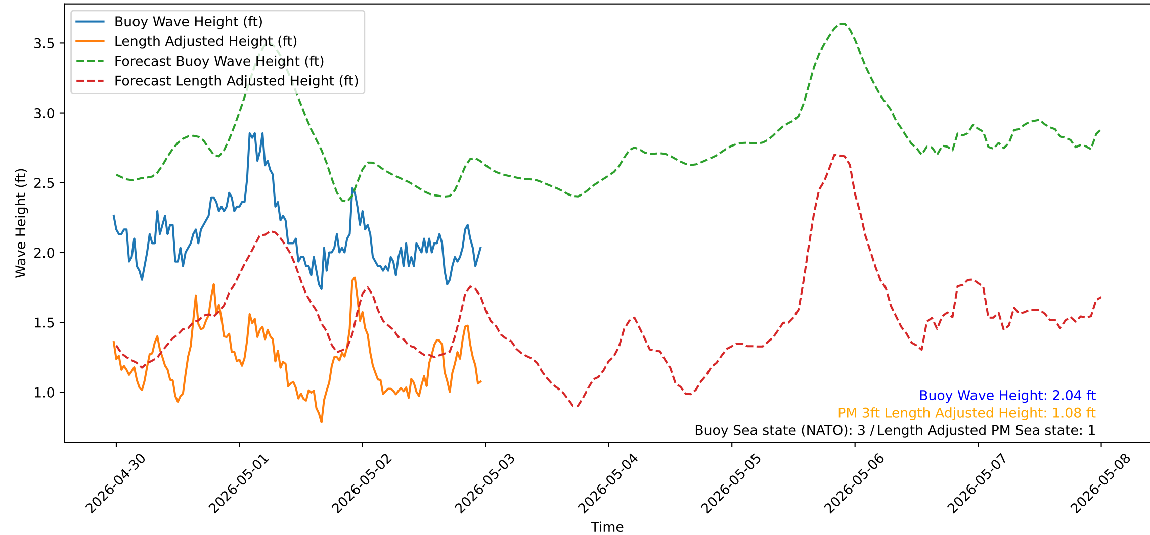
Wave Heights over Time for Green Beach at 2026-05-02 23:41:13
