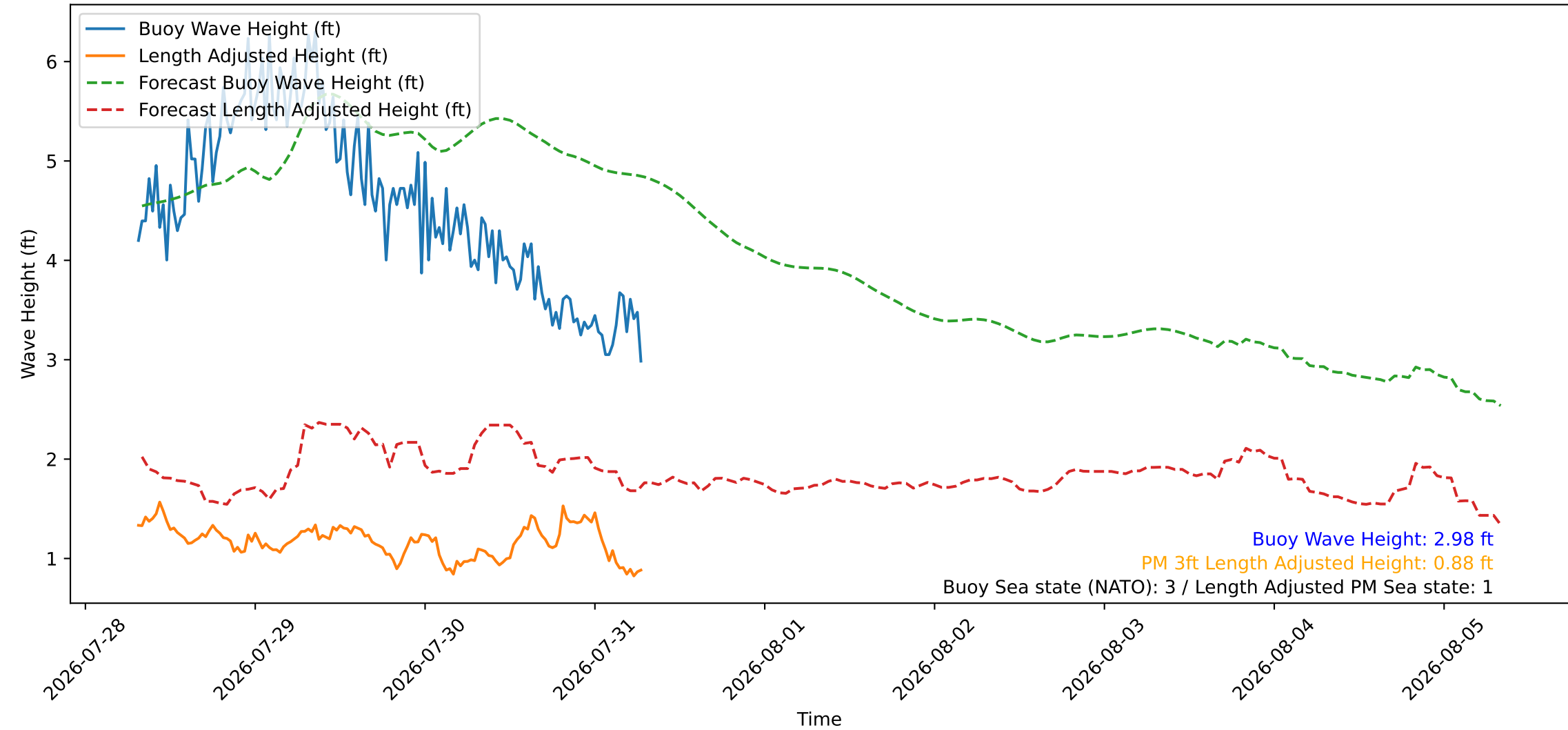
Wave Heights over Time for Green Beach at 2026-07-31 07:31:09
