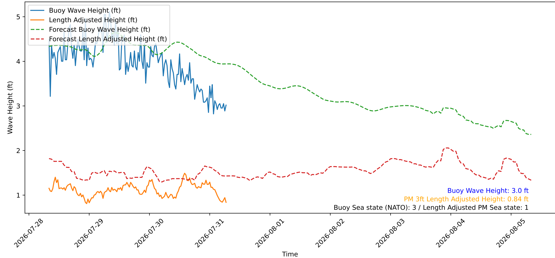
Wave Heights over Time for Red Beach at 2026-07-31 07:30:46
