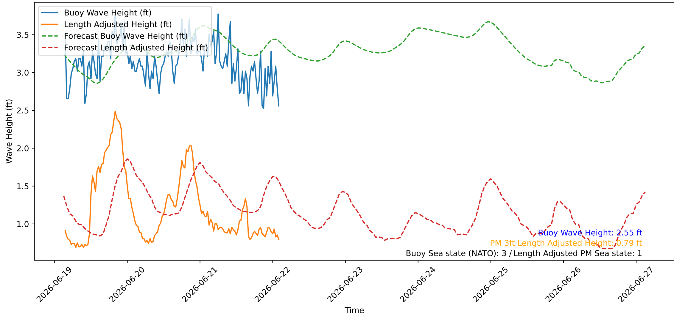
Wave Heights over Time for Red Beach at 2026-06-22 03:00:45
