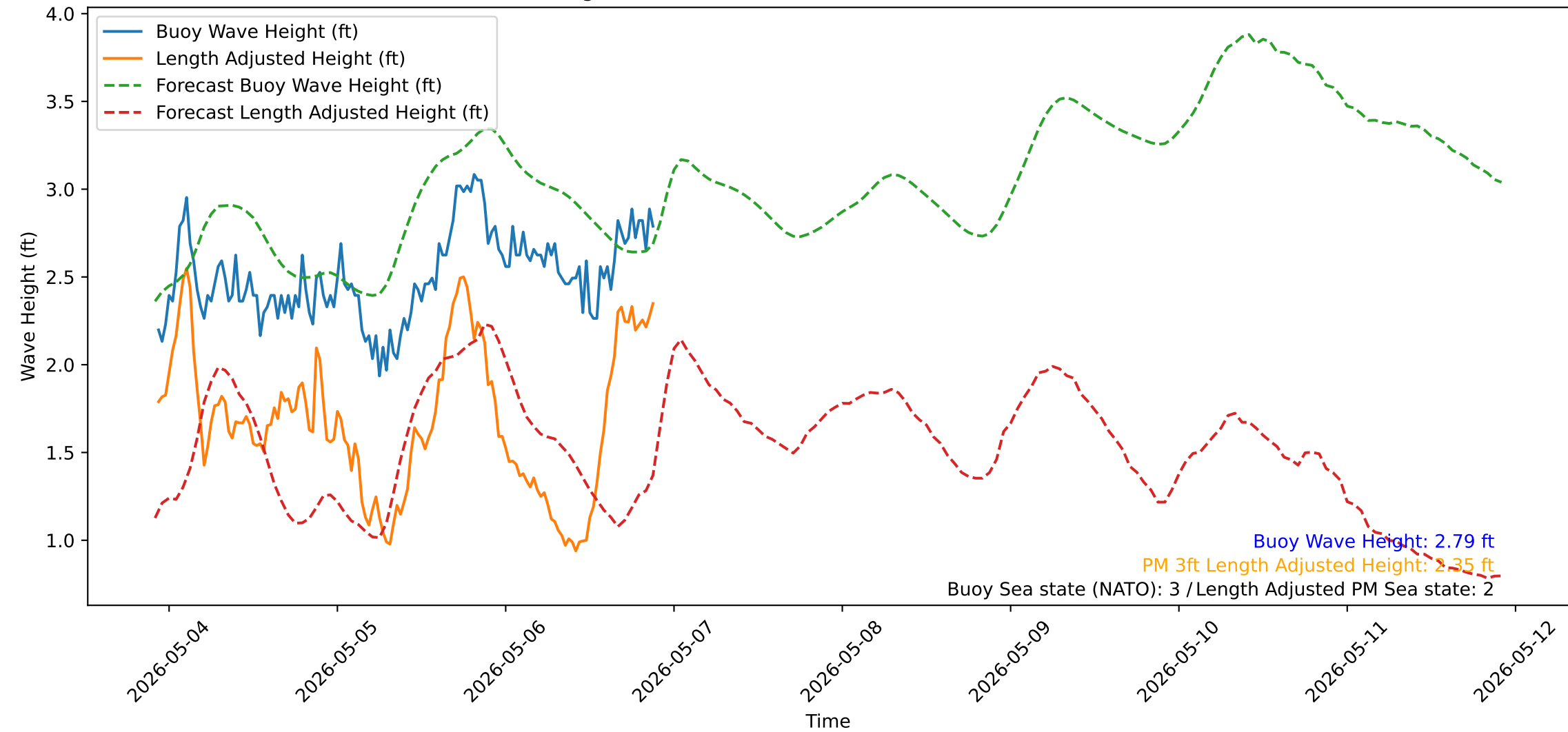
Wave Heights over Time for Red Beach at 2026-05-06 22:20:51
