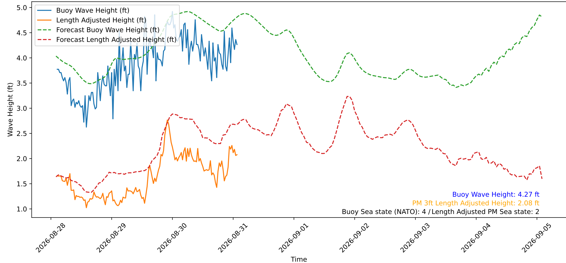
Wave Heights over Time for Green Beach at 2026-08-31 02:21:14
