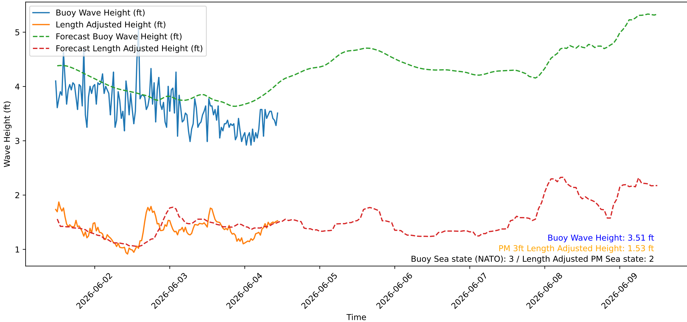
Wave Heights over Time for Oceanside Harbor at 2026-06-04 11:30:26
