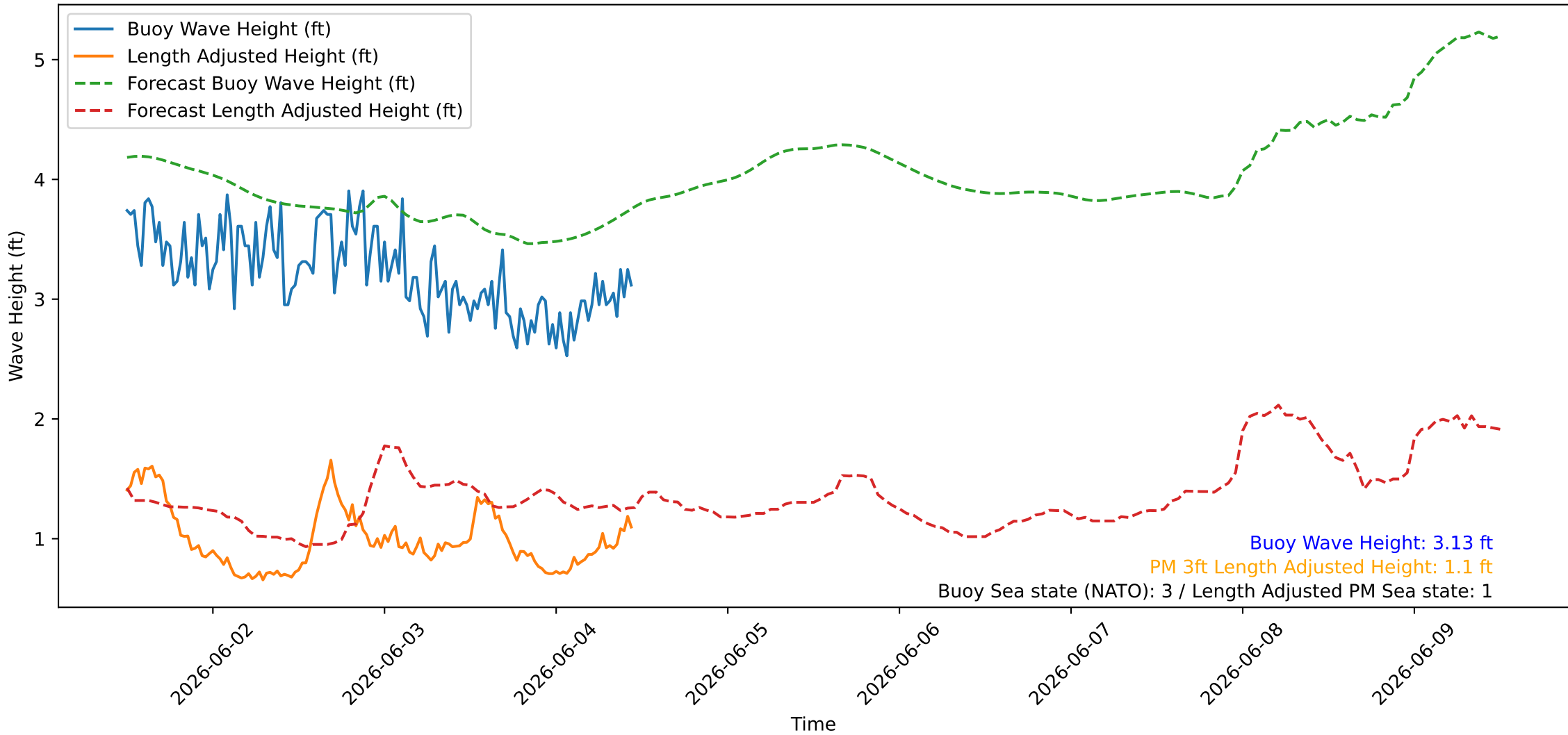
Wave Heights over Time for Red Beach at 2026-06-04 11:30:45
