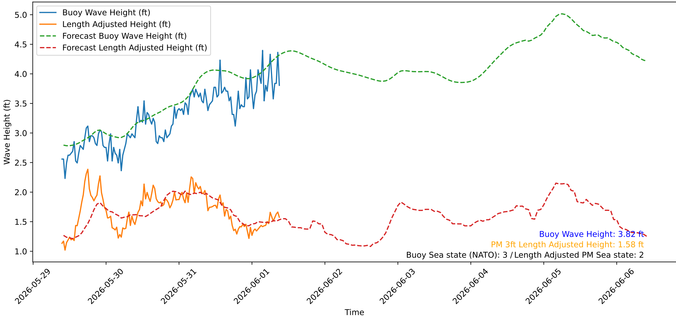
Wave Heights over Time for Oceanside Harbor at 2026-06-01 09:40:26
