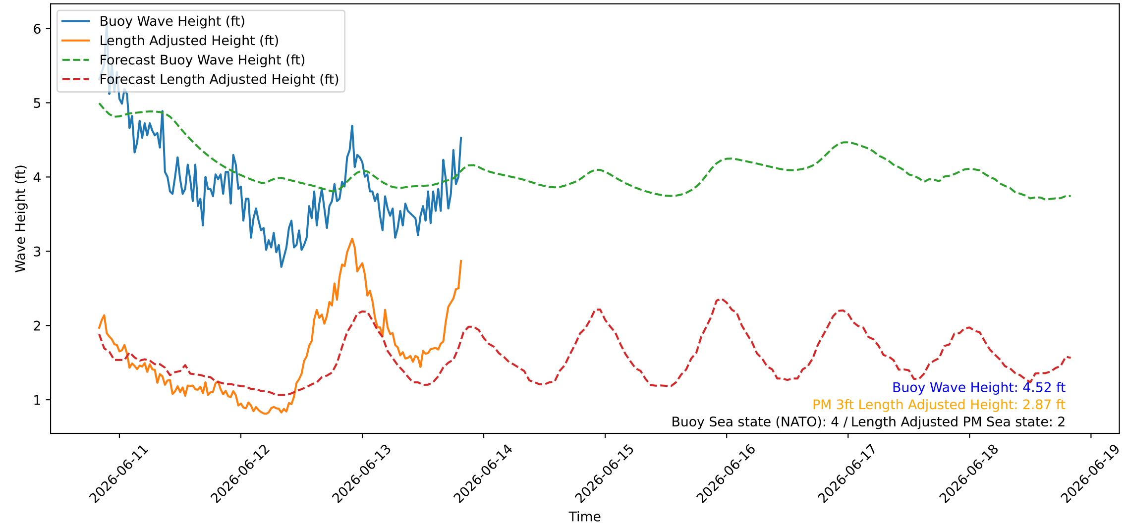
Wave Heights over Time for Oceanside Harbor at 2026-06-13 20:10:27
