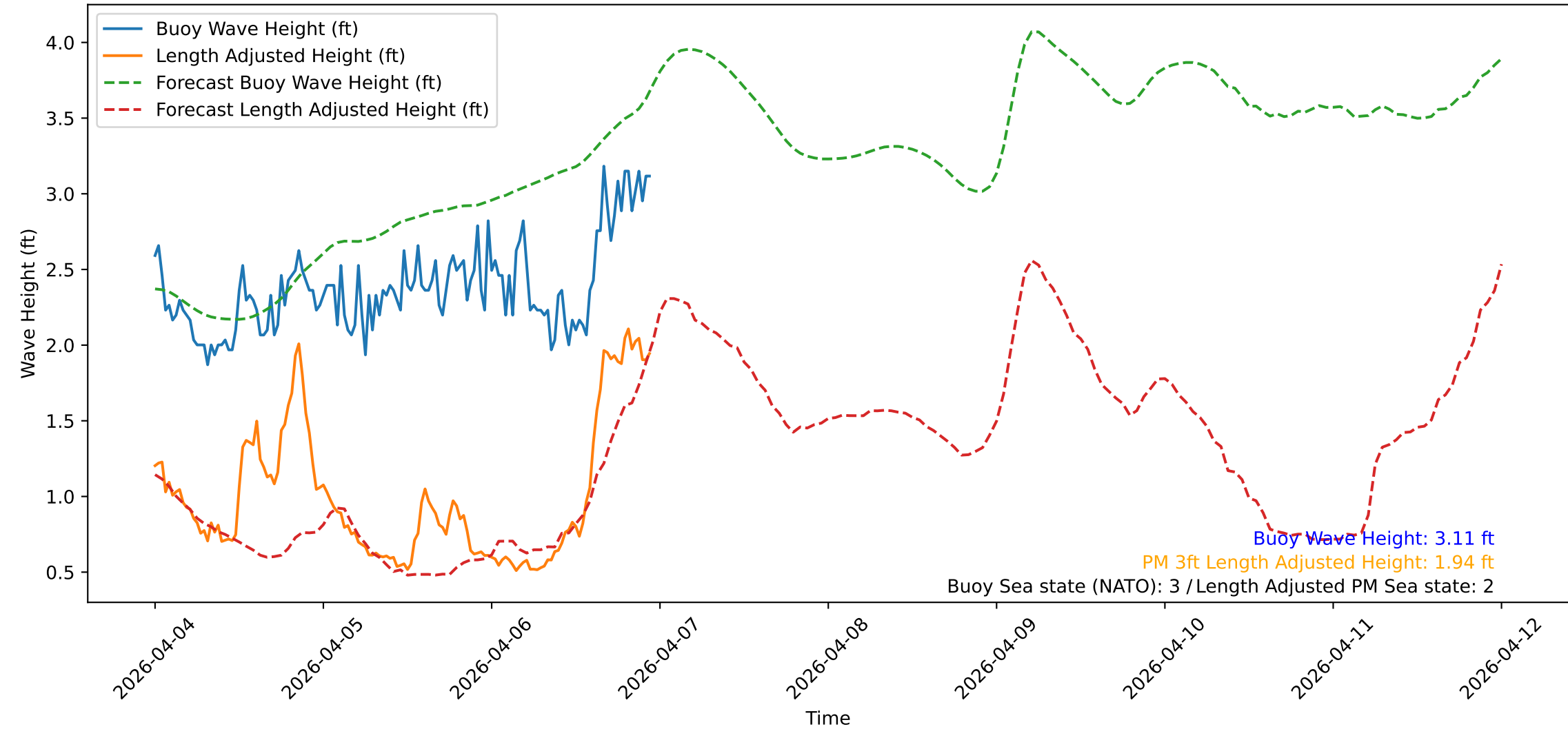
Wave Heights over Time for Red Beach at 2026-04-06 23:40:47
