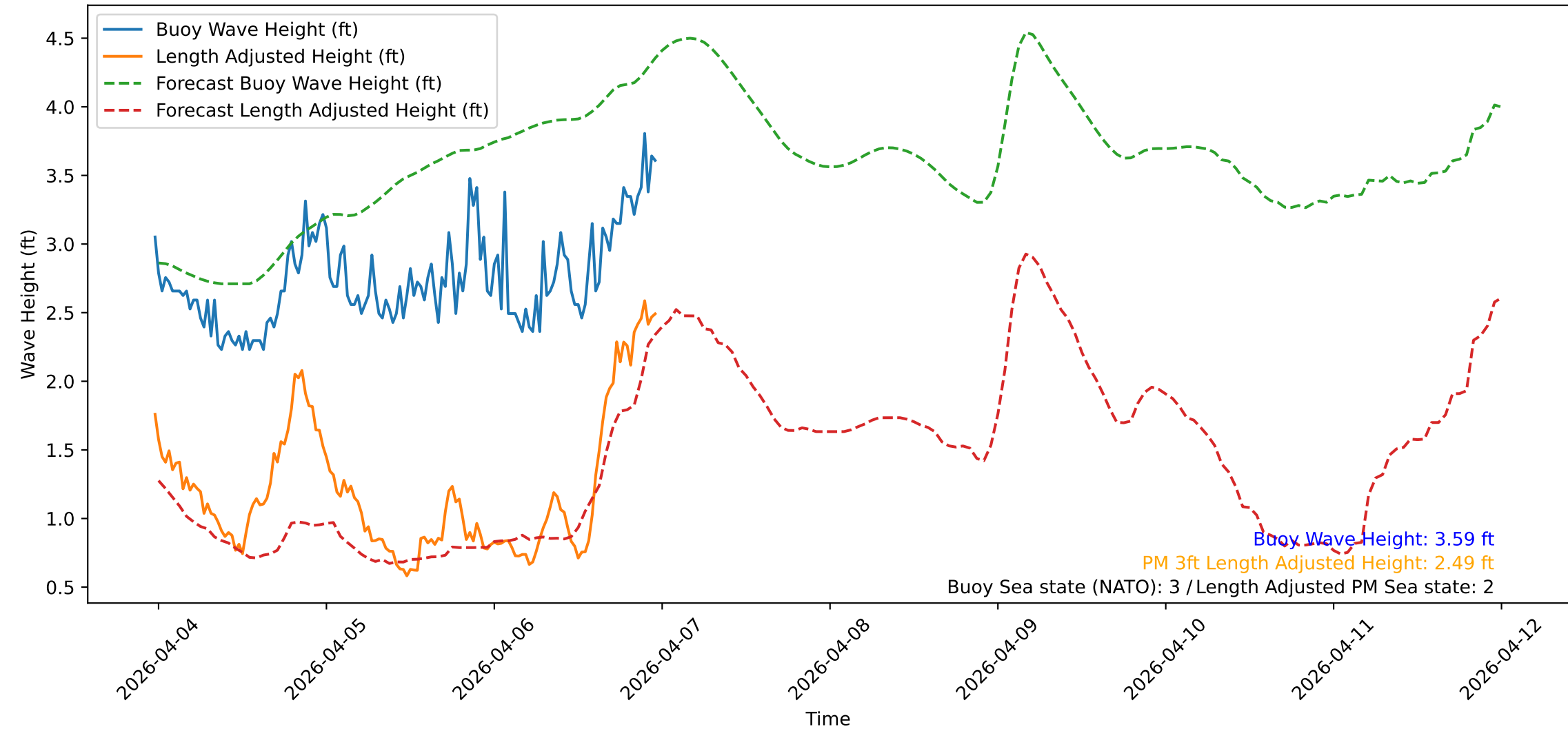
Wave Heights over Time for Green Beach at 2026-04-06 23:41:10
