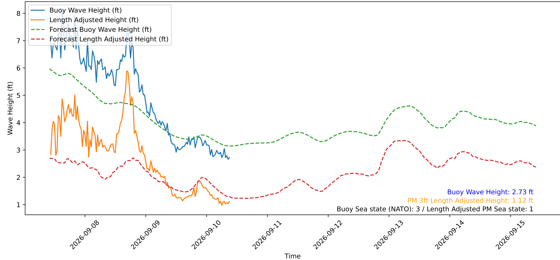
Wave Heights over Time for Green Beach at 2026-09-10 10:01:12
