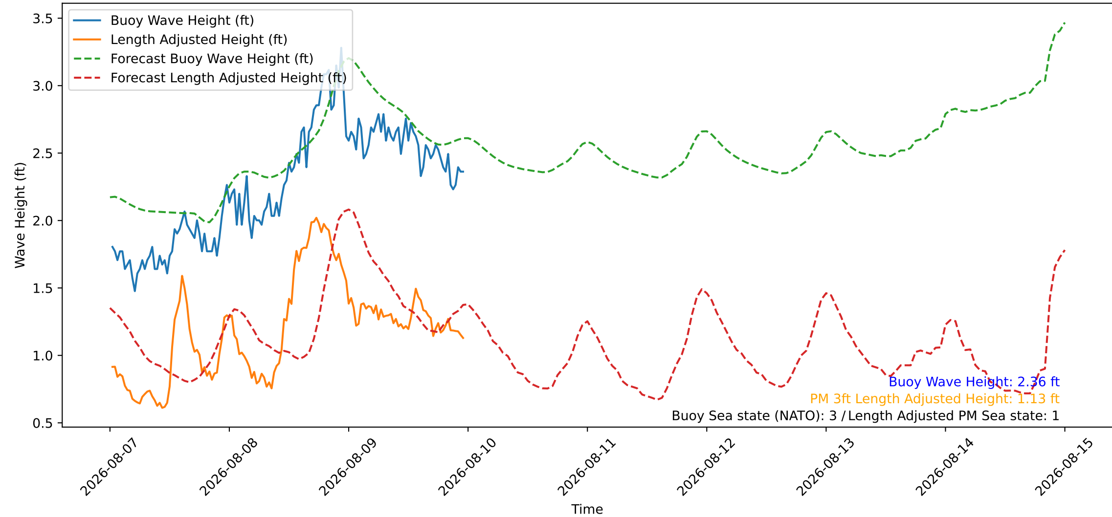
Wave Heights over Time for Red Beach at 2026-08-10 00:00:46
