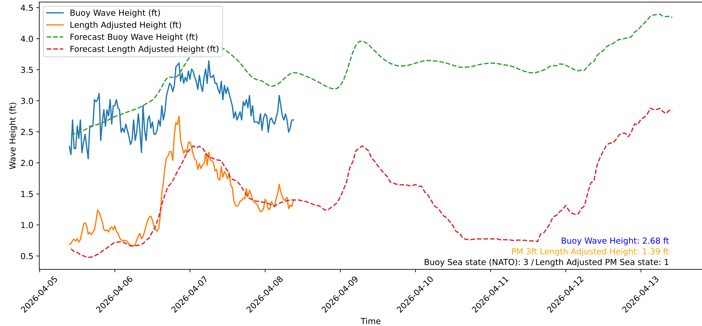
Wave Heights over Time for Oceanside Harbor at 2026-04-08 09:40:34
