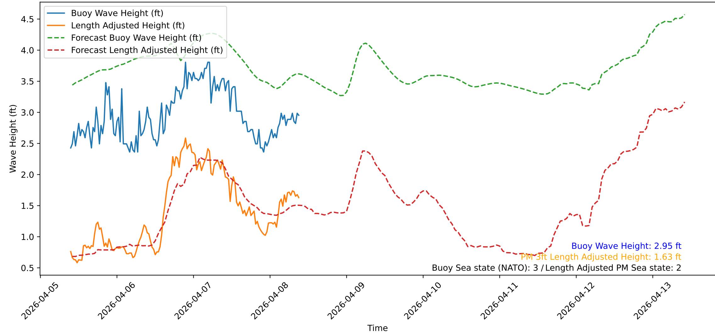
Wave Heights over Time for Green Beach at 2026-04-08 09:41:12
